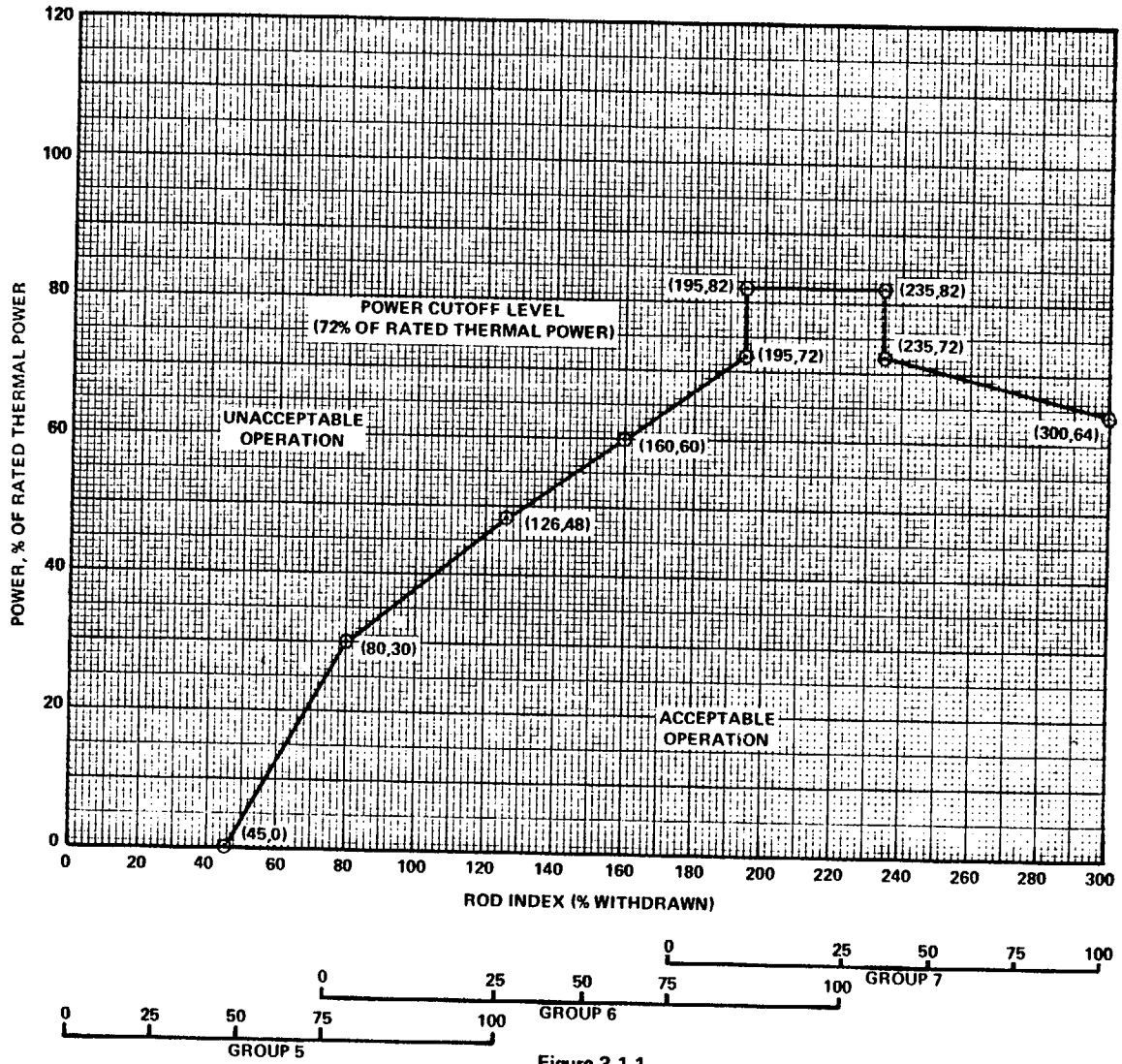
Figure 3.1-1 Regulating Rod Group Insertion Limits for 4 Pump Operation up to Control Rod Interchange 250 \pm 10 EFPD
