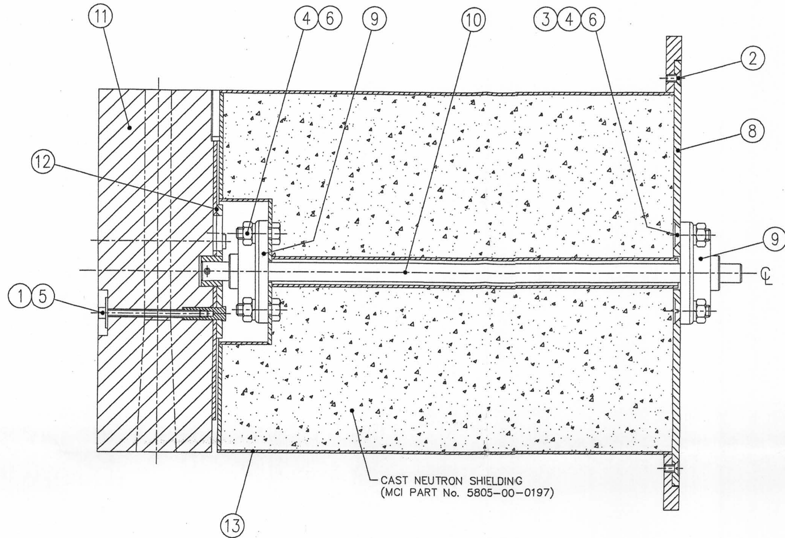
SECTION ON C-C
