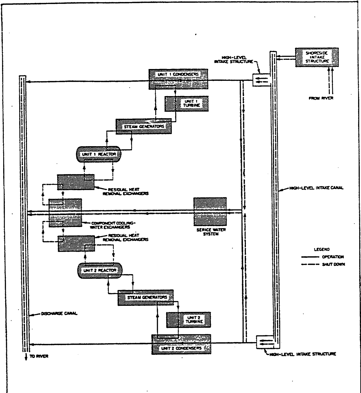
FIGURE 9: Simplified flow diagram of the heat dissipation system at the Surry Power Station
