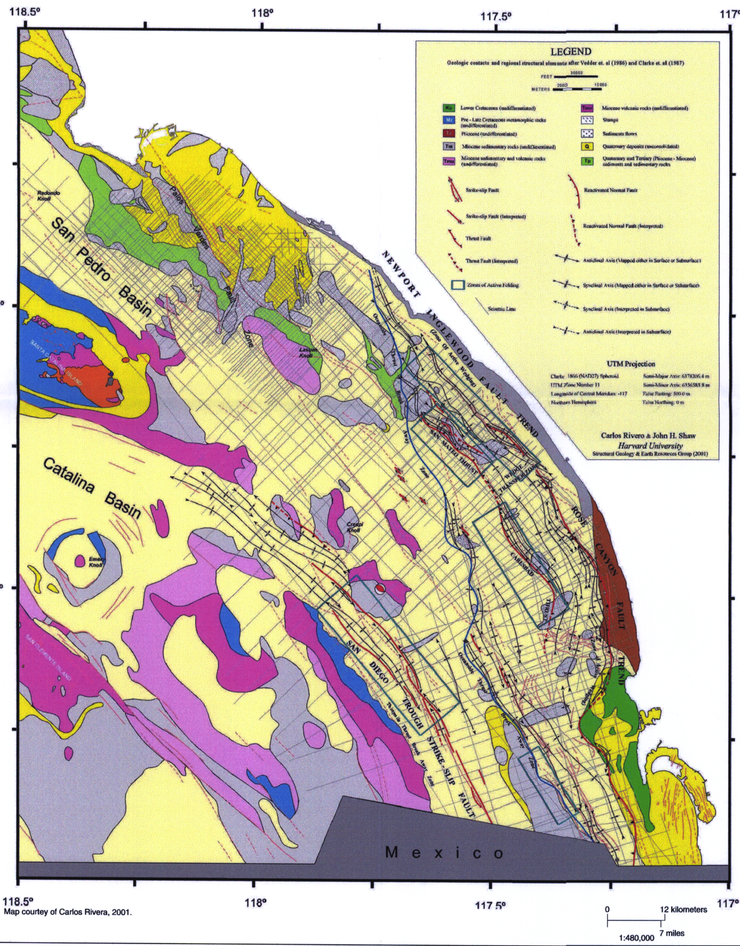
FAULTING AND FOLDING OF COVER SEDIMENTS (OFFSHORE REGION) (Rivero & Shaw, 2001)
