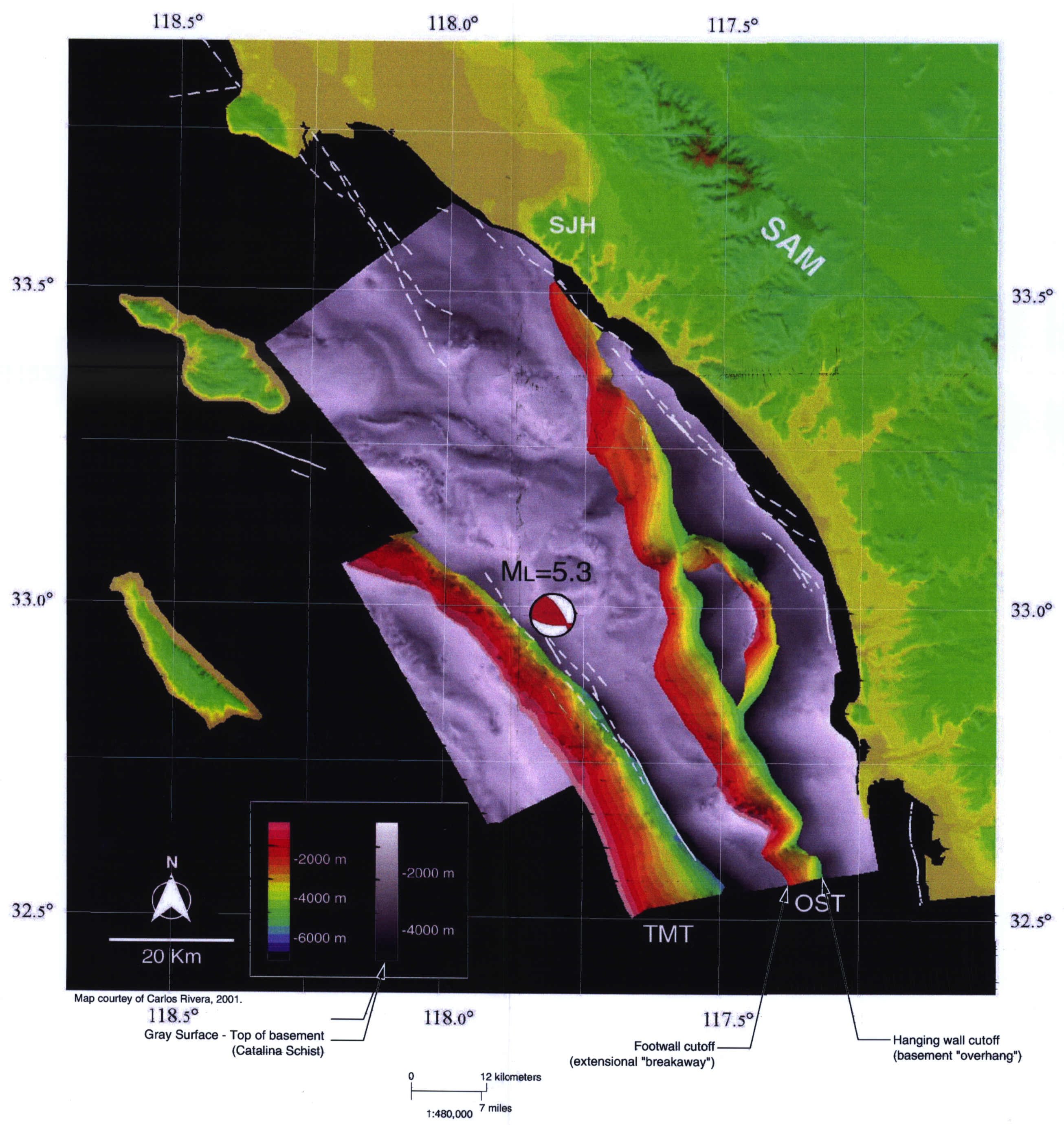
FAULTING OF BASEMENT (OFFSHORE REGION) (Rivero & Others, 2000)
