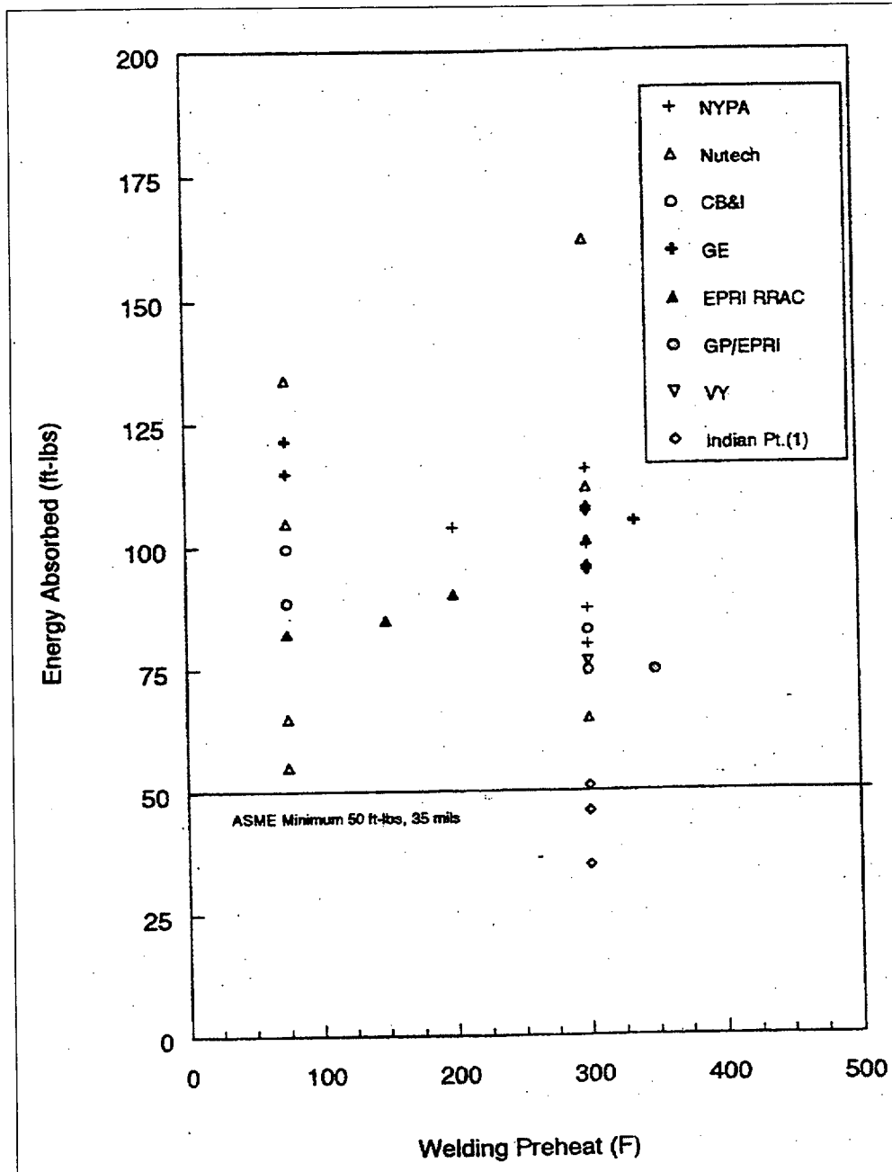
Figure 4-2 HAZ Toughness Data from Various Industry Qualifications on RPV Steels. (Note 1—Under an USNRC Relief Request, Indian Point was qualified to 30 ft-lbs minimum.)
