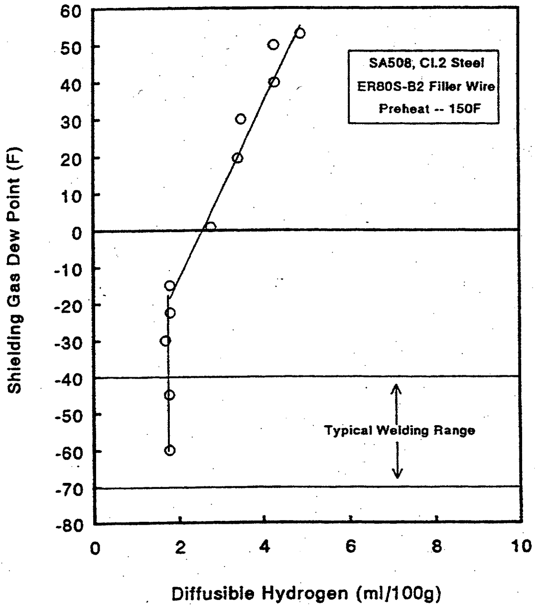
Figure 4-1 Diffusible Hydrogen Levels at Various Shielding Gas Dewpoint Temperatures
