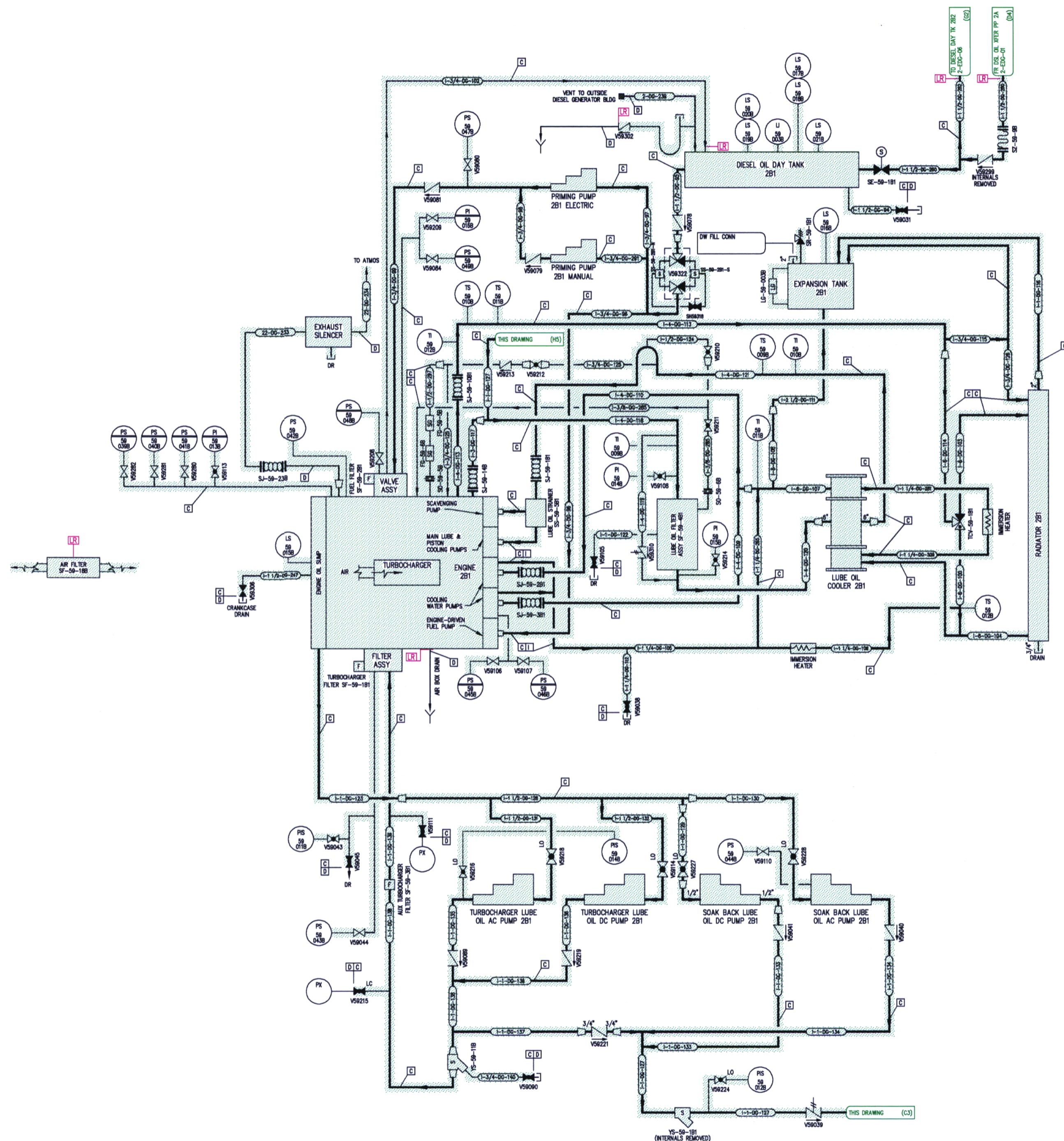
DIESEL GENERATOR 2B1 (16-CYL)
