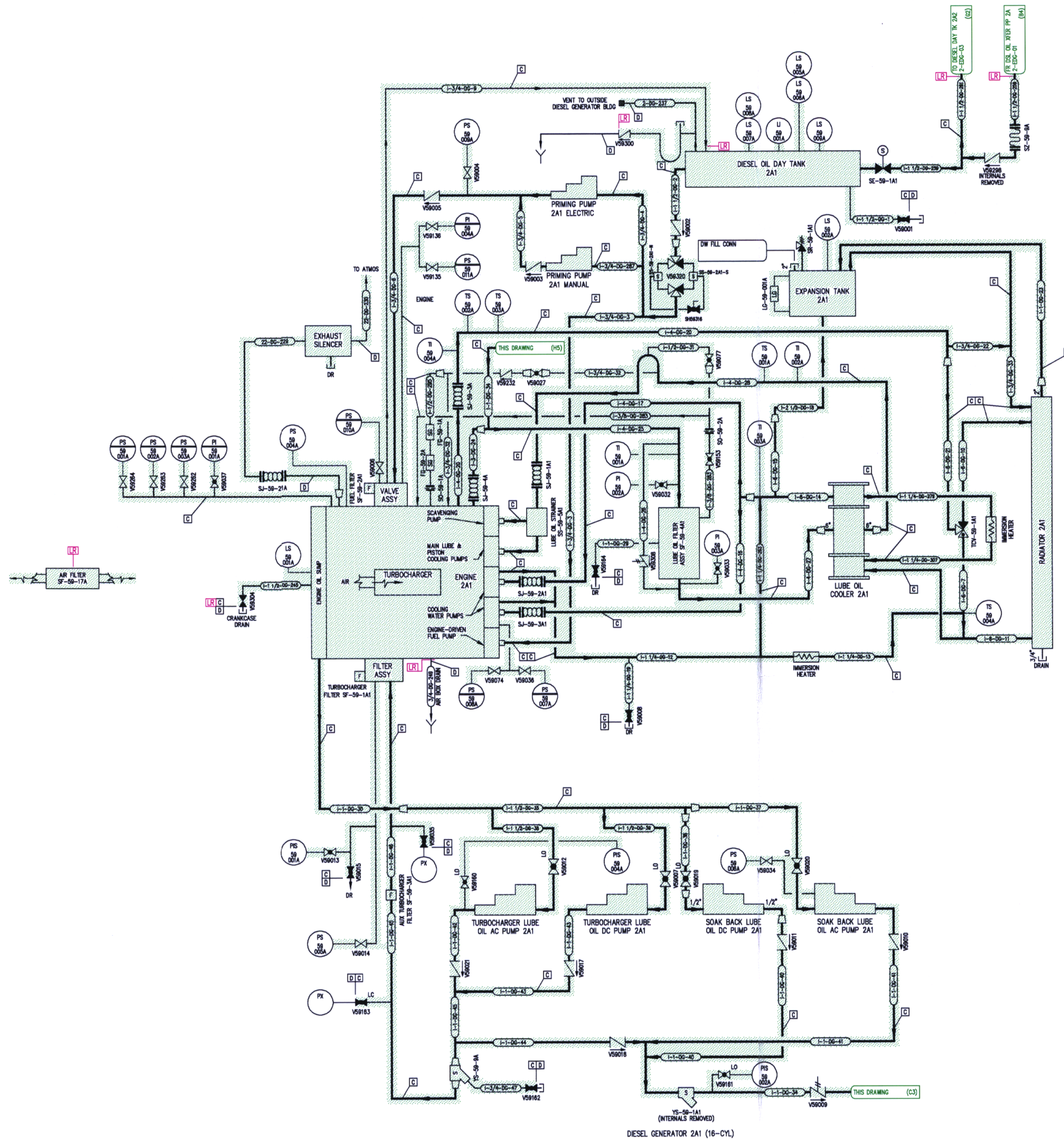
DIESEL GENERATOR 2A1 (16-CYL)
