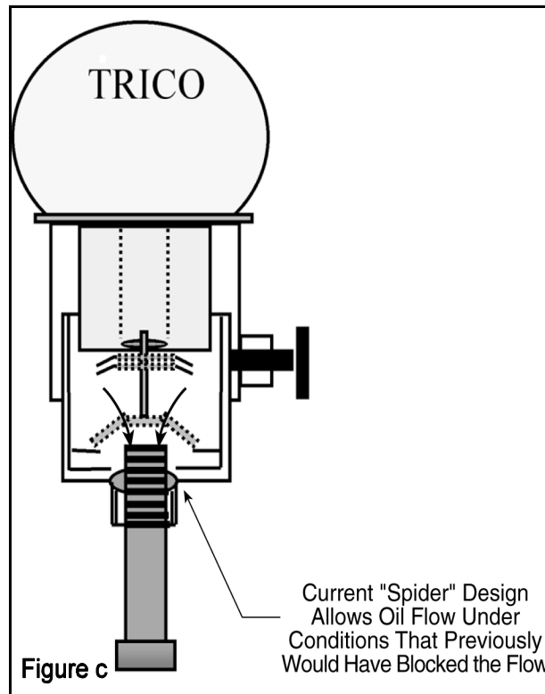
Trico Opto-Matic Oil Bubbler
