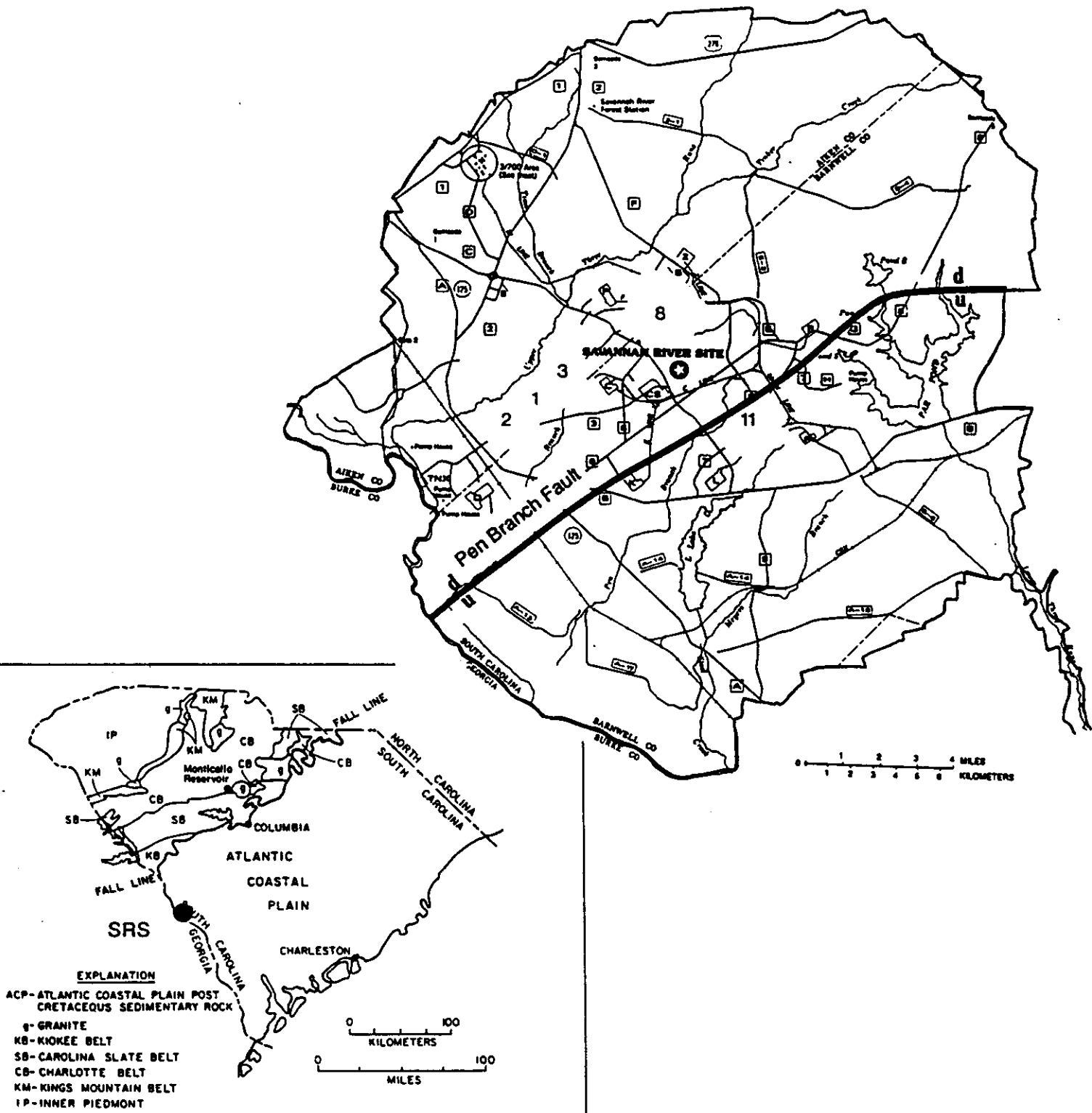
Figure 1 Geologic map of South Carolina, showing the location of the Savannah River Site (SRS) along the Savannah River southeast of Augusta, GA. Also shown is a map of the SRS showing the locations of the boreholes mentioned in this report. Numbers refer to SSW-1, SSW-2, SSW-3, DRB-8 and DRB-11 previously studied; the star shows the location of the NPR Hole. The approximate location of the NE-SW trending Pen Branch Fault, which bounds the Dunbarton Basin along its NW edge, is shown by the dark line (u on upthrown side of fault).
