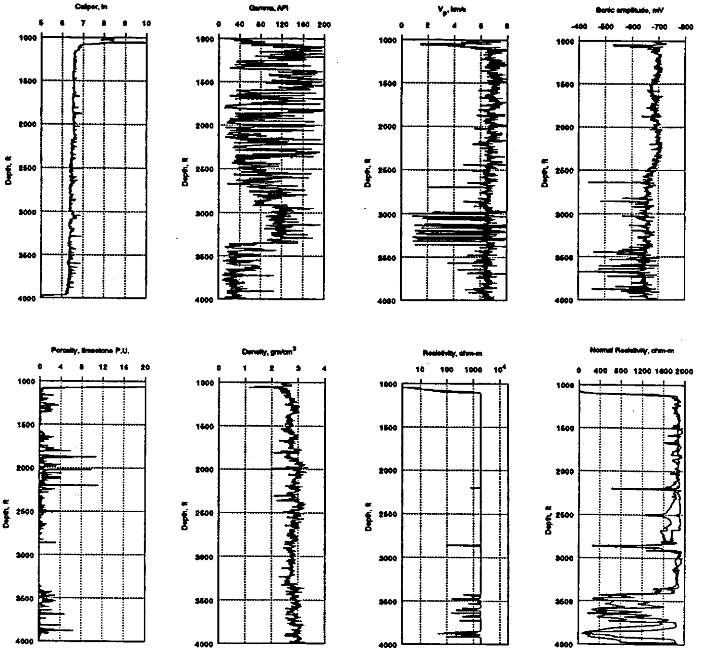
Figure 7 Geophysical logs recorded by the US Geological Survey (courtesy of Jerry Idler, U.S.G.S. Doreville, GA) in the NPR Hole.
