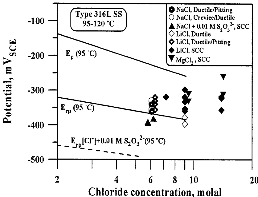
Figure 3: Slow strain rate test results for type 316L SS in various chloride solutions. E_p and E_{rp} denote the pit initiation potential and the repassivation potential.
