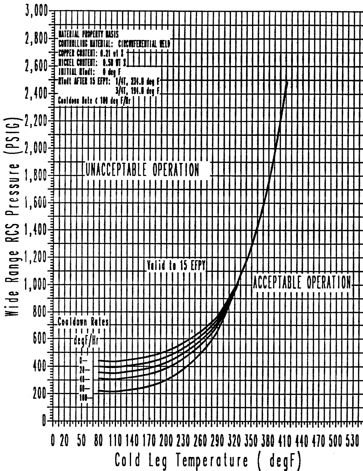
Figure 3.1-2 RCS Cooldown Limitations
