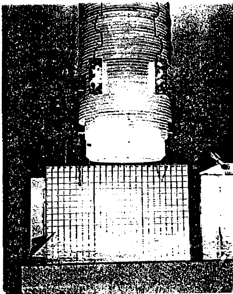
Figure 4/1 Pre-Drop 4 - The Basket suspended at the drop altitude 60 inches above the target
