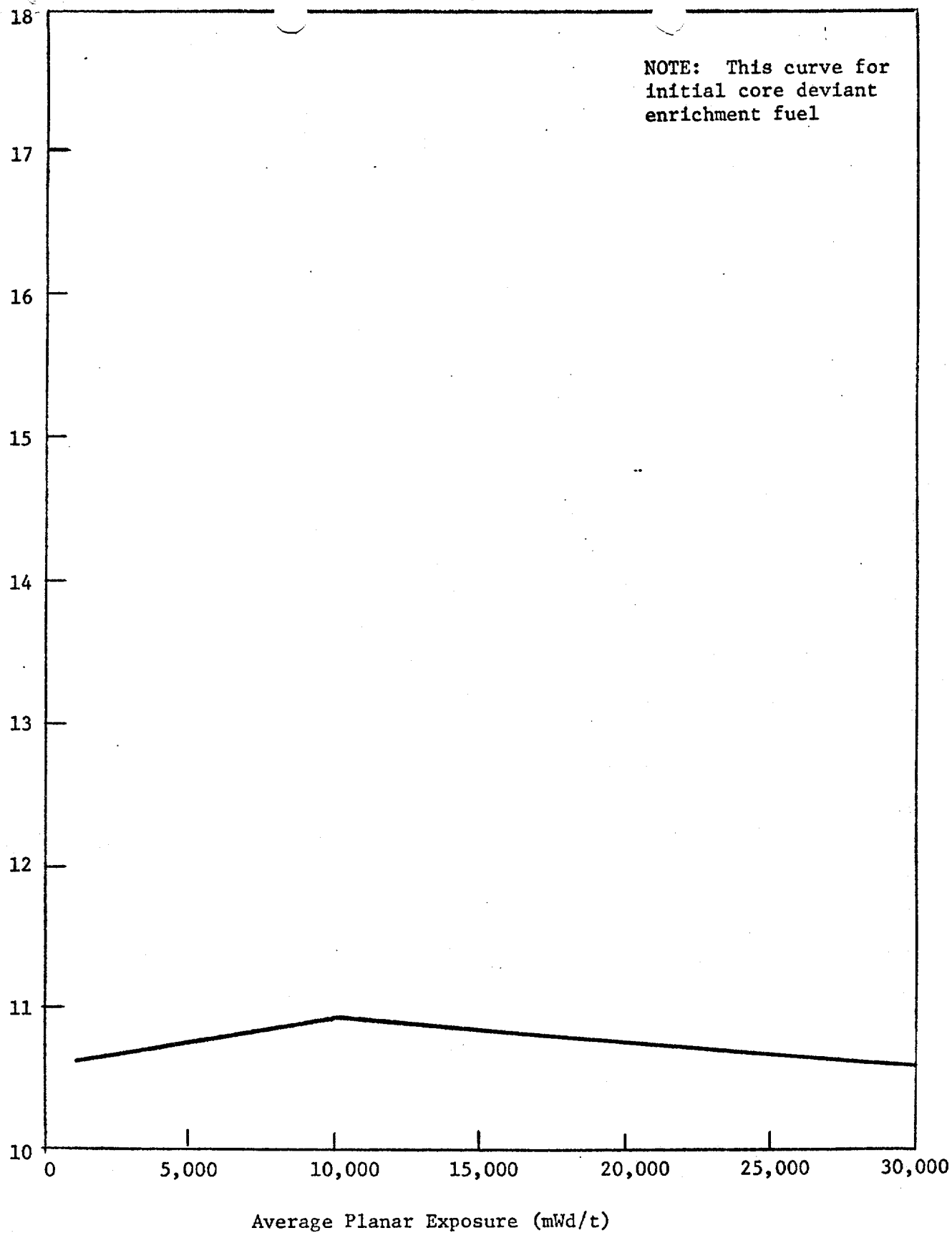
FIGURE 3.5.1A MAXIMUM ALLOWABLE PLANAR LHGR
