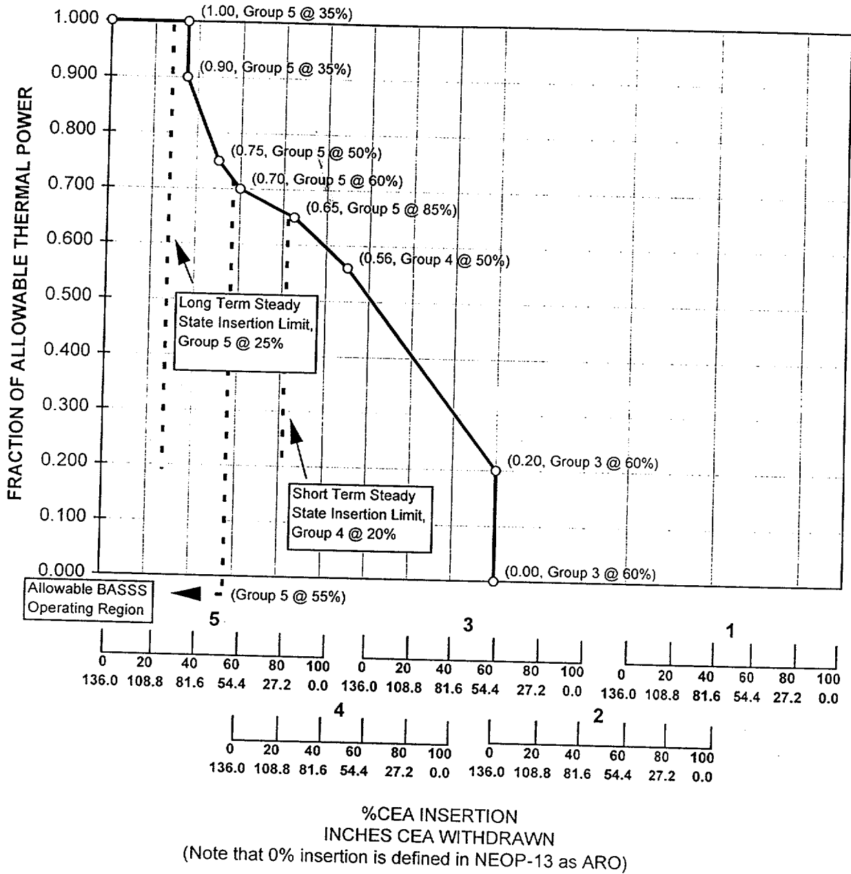
Figure 3.1.6 CEA Group Insertion Limits vs. Fraction of Rated Thermal Power
