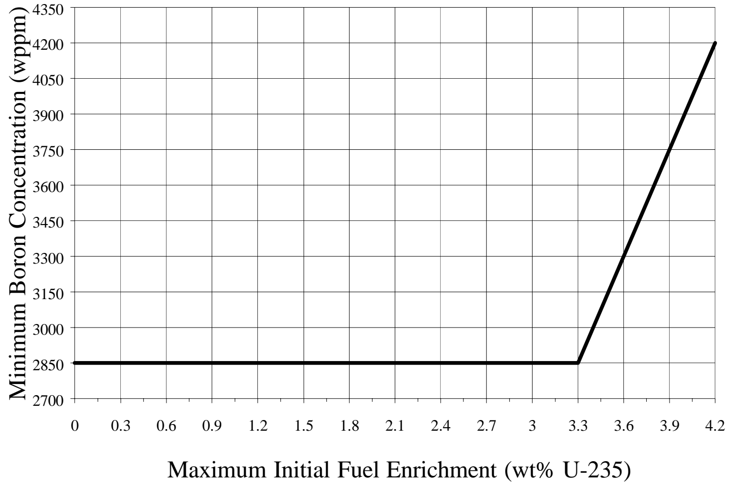
Figure 2 B&W 15x15 Fuel Boron Concentration Curve
