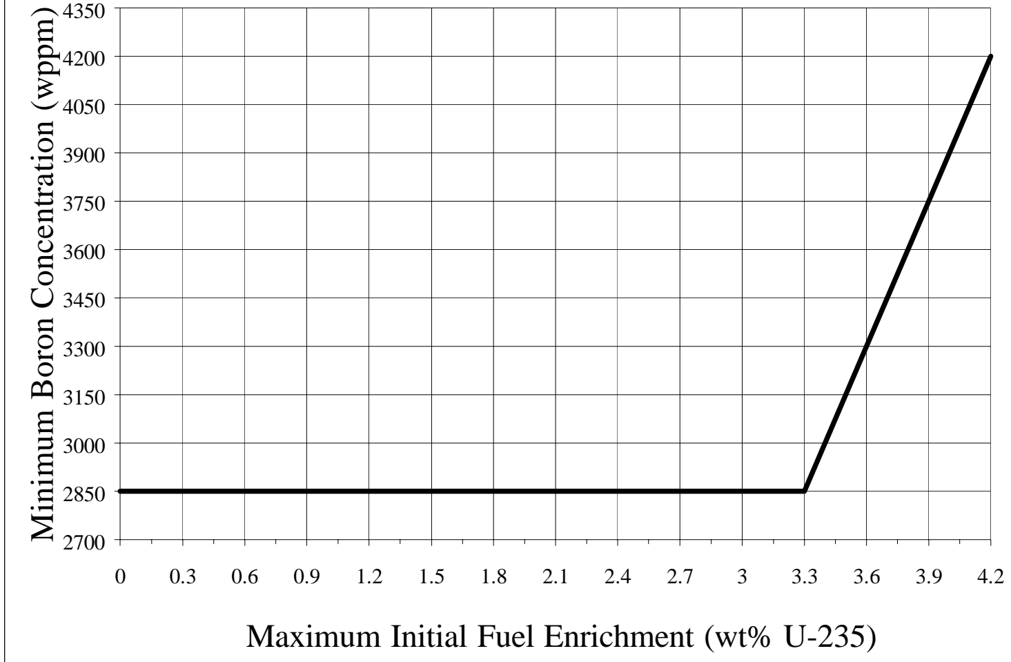
Figure 2 B&W 15x15 Fuel Boron Concentration Curve
