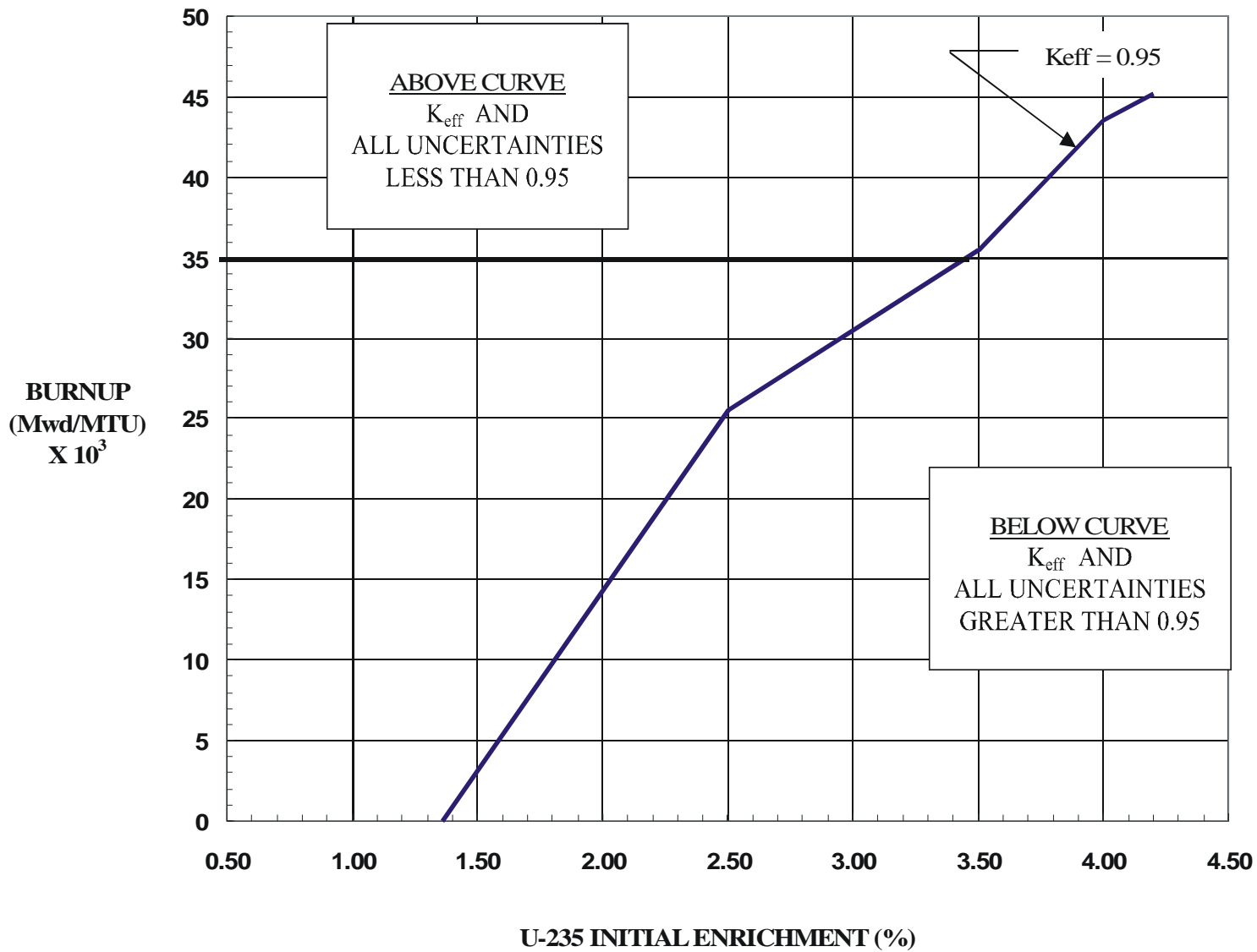
FUEL CRITICALITY ACCEPTABILITY CURVE
