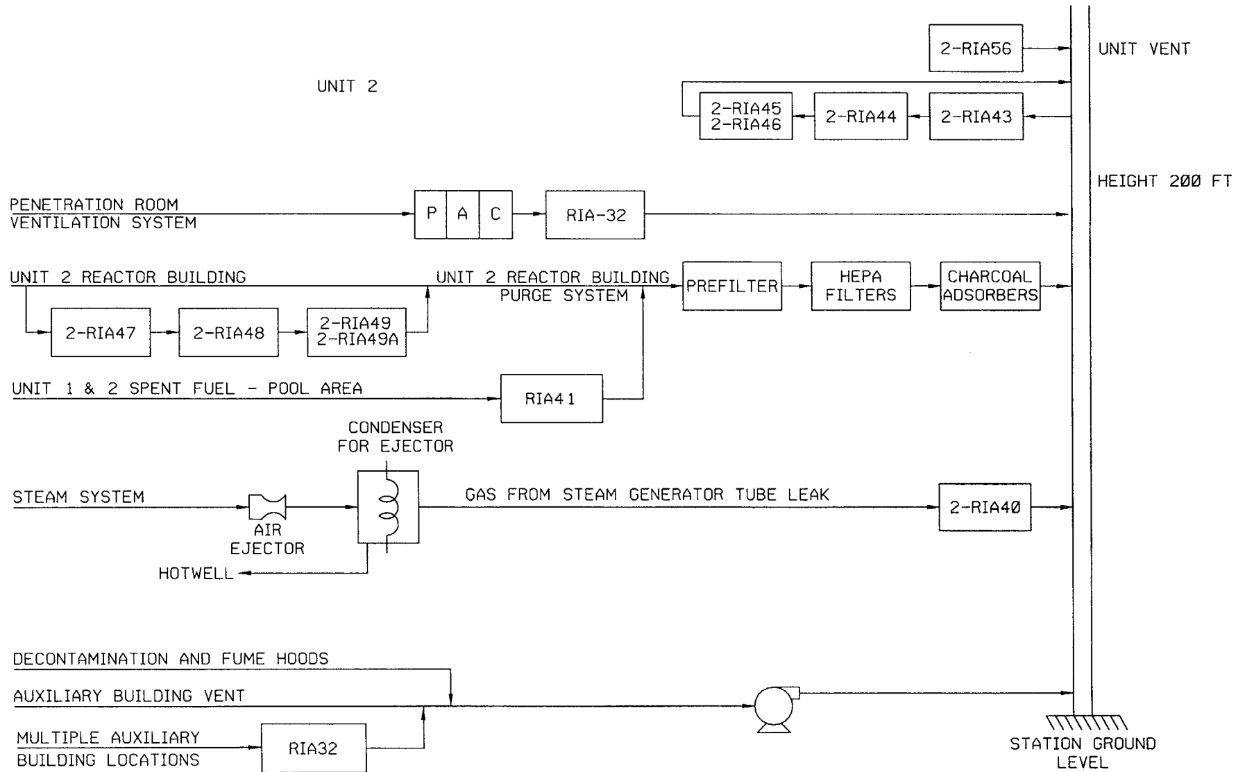
Figure 1.0-2 Dconee Nuclear Station Gaseous Radwaste System Page 2 of 4
