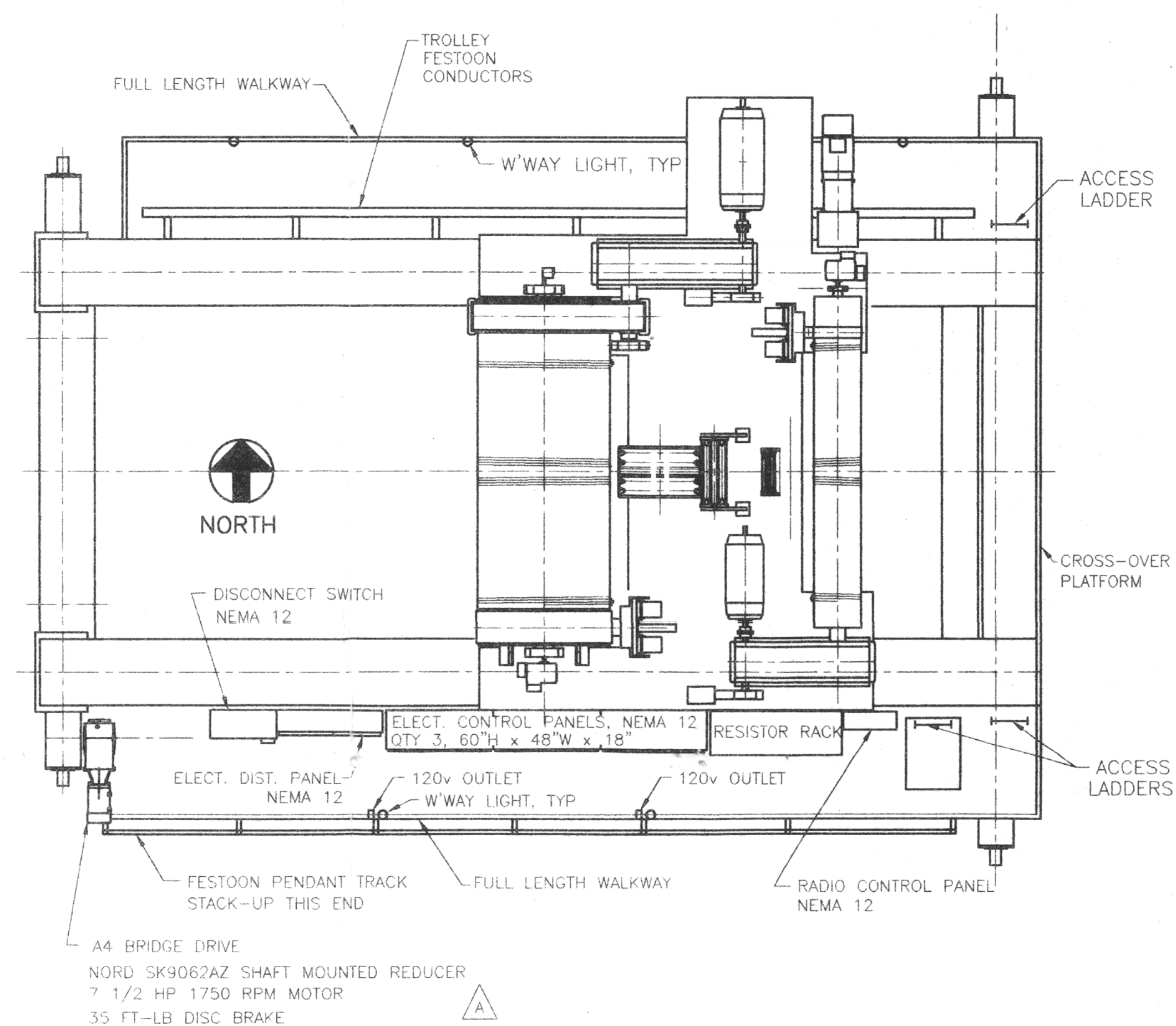
PLAN VIEW
