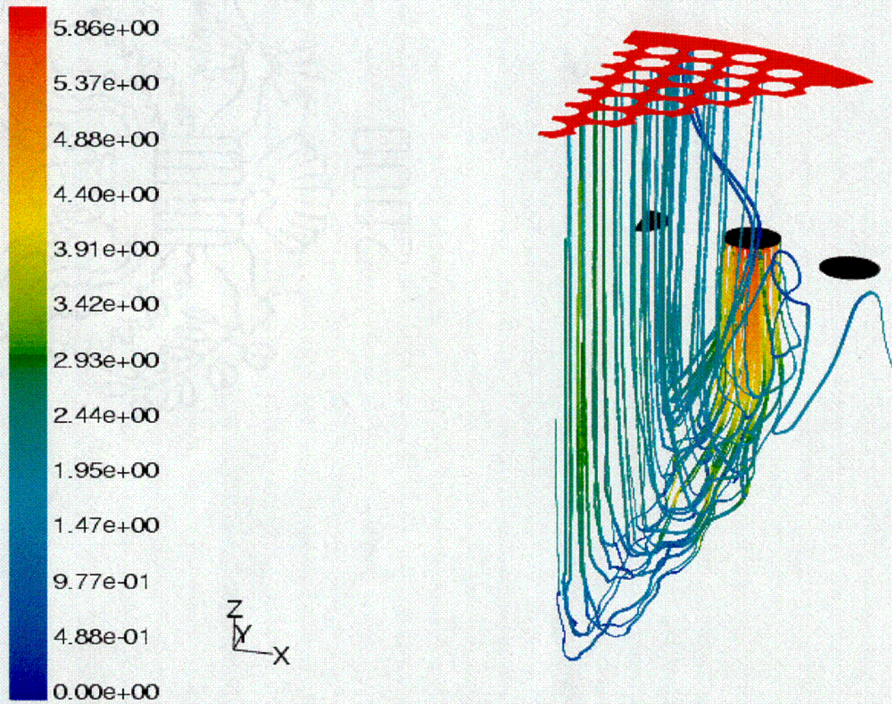
Path Lines Colored by Velocity Magnitude (m/s) Dec 21, 2000 FLUENT 5.4 (3d, dp, segregated, rngke)
