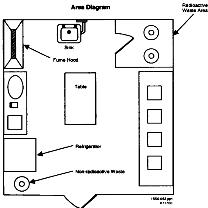
Figure P.1 Area Diagram. This is an example of a laboratory survey map.
