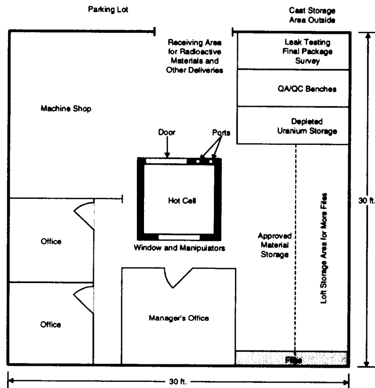
Figure 8.7 Facility Diagram for a Radiography Source Manufacturer.
