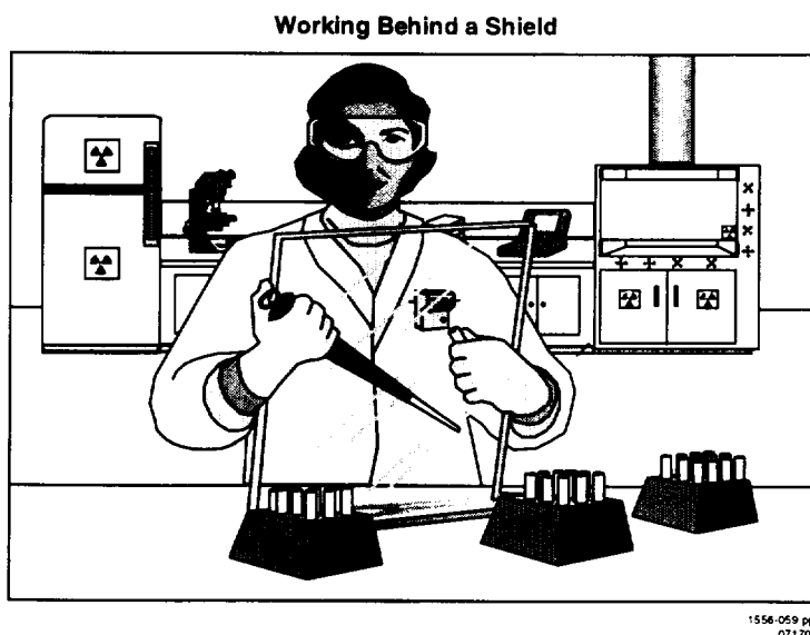
Figure 8.13 Use of Appropriate Shielding. This worker is using high density plastic shielding, which is appropriate for radioisotopes that emit beta radiation.
