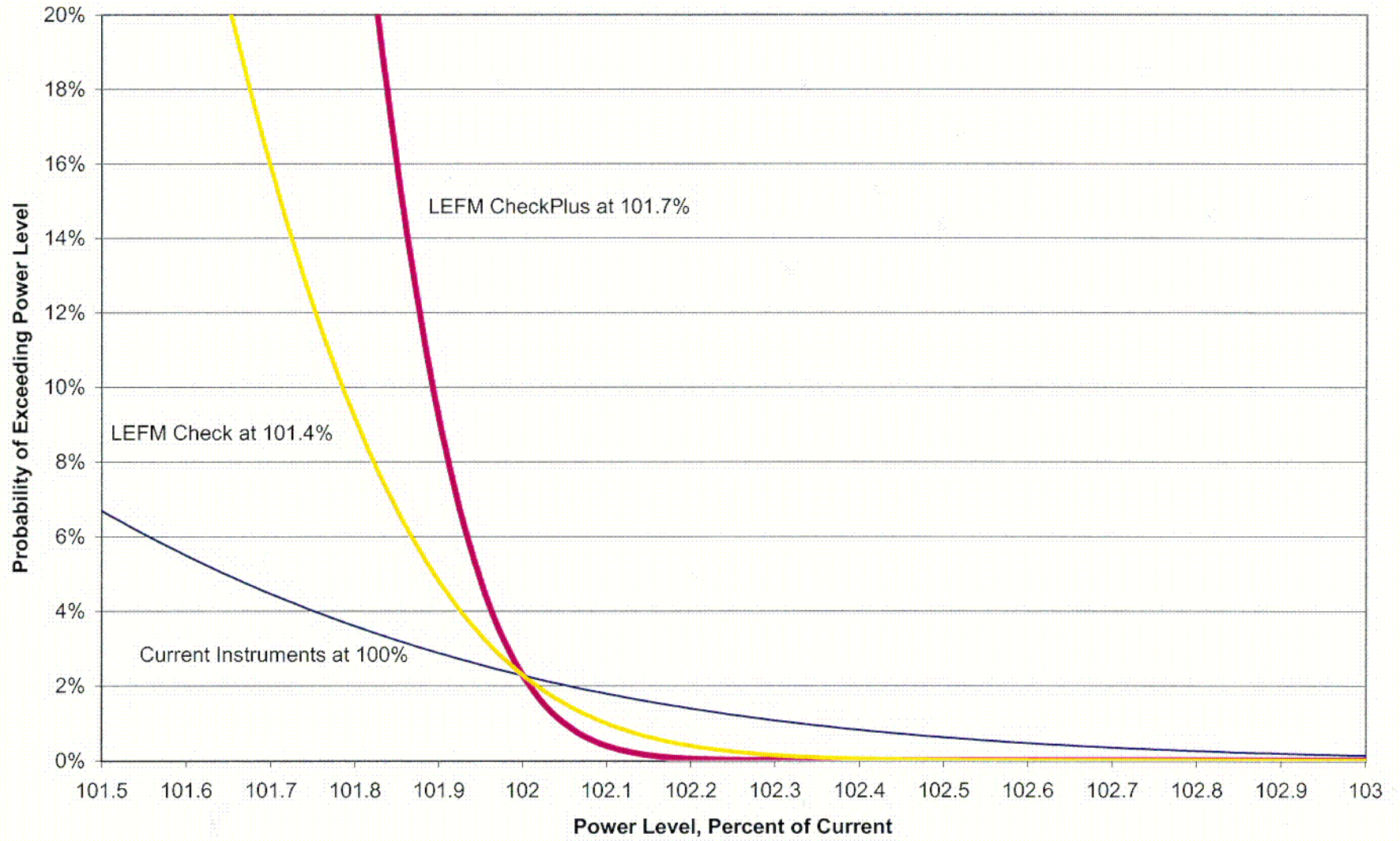
Figure 3. Probability of Exceeding Power Level in the Vicinity of 102% Power
