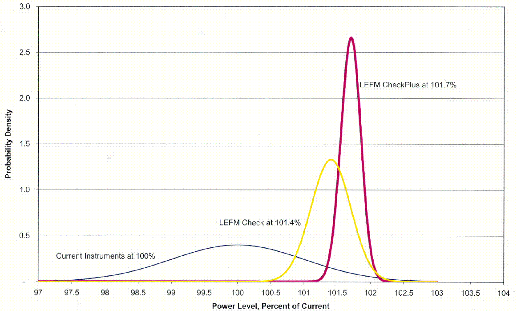
Figure 1. Probable Operating Ranges For LEFM Systems at Increased Power Levels
