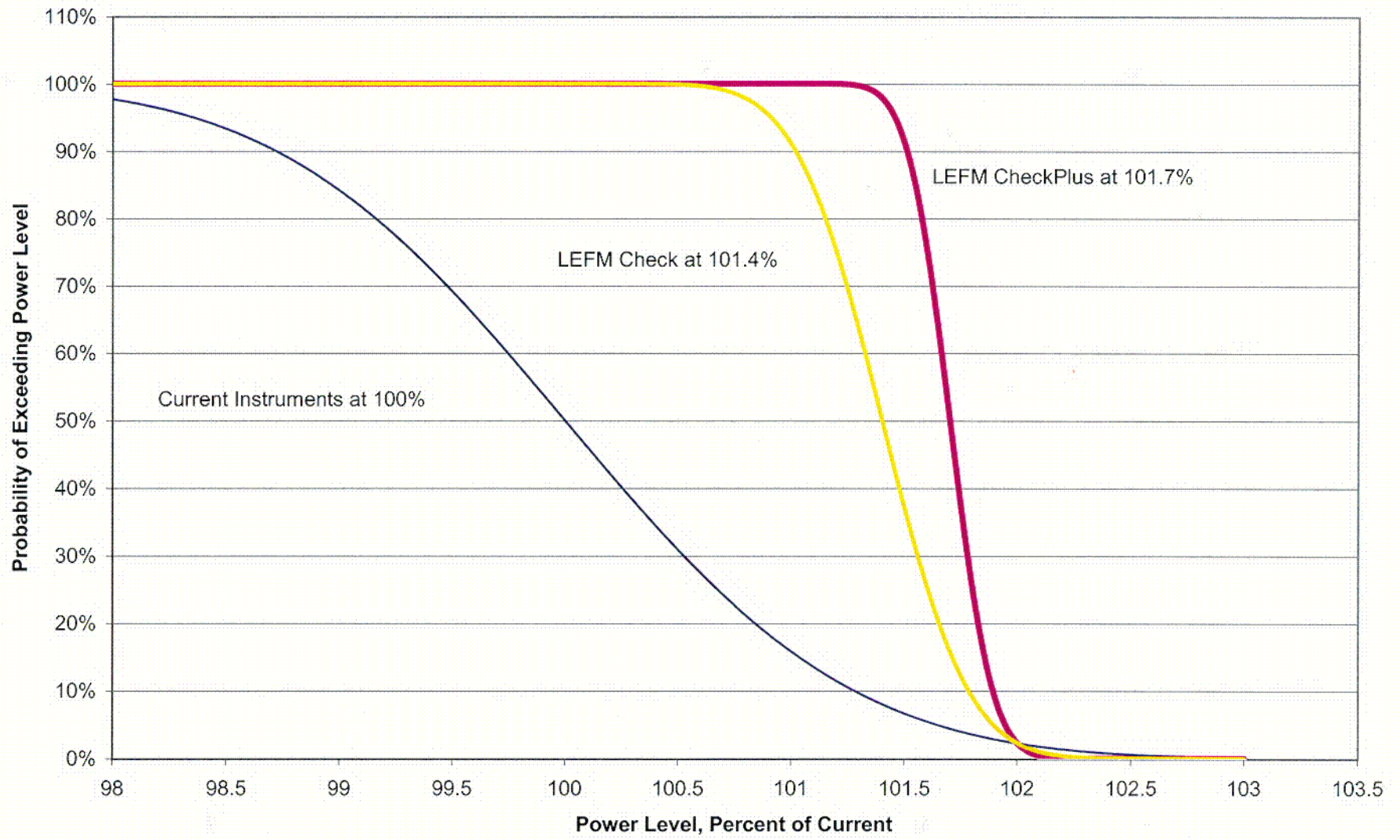
Figure 2. Probability of Exceeding Power Levels With LEFM Systems And Increased Power
