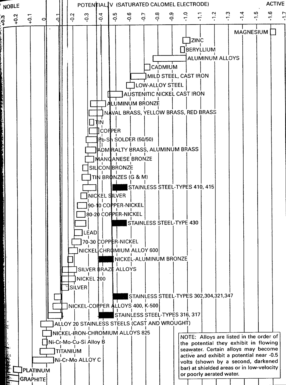
Figure 6.7—Galvanic Series of Various Metals and Alloys in Seawater
