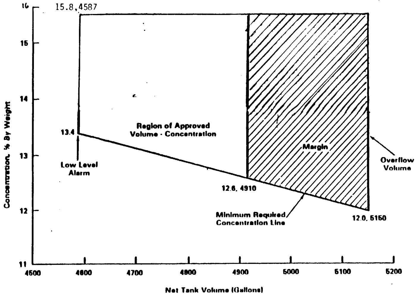
FIGURE 3.1.5-2 SODIUM PENTABORATE SOLUTION CONCENTRATION
