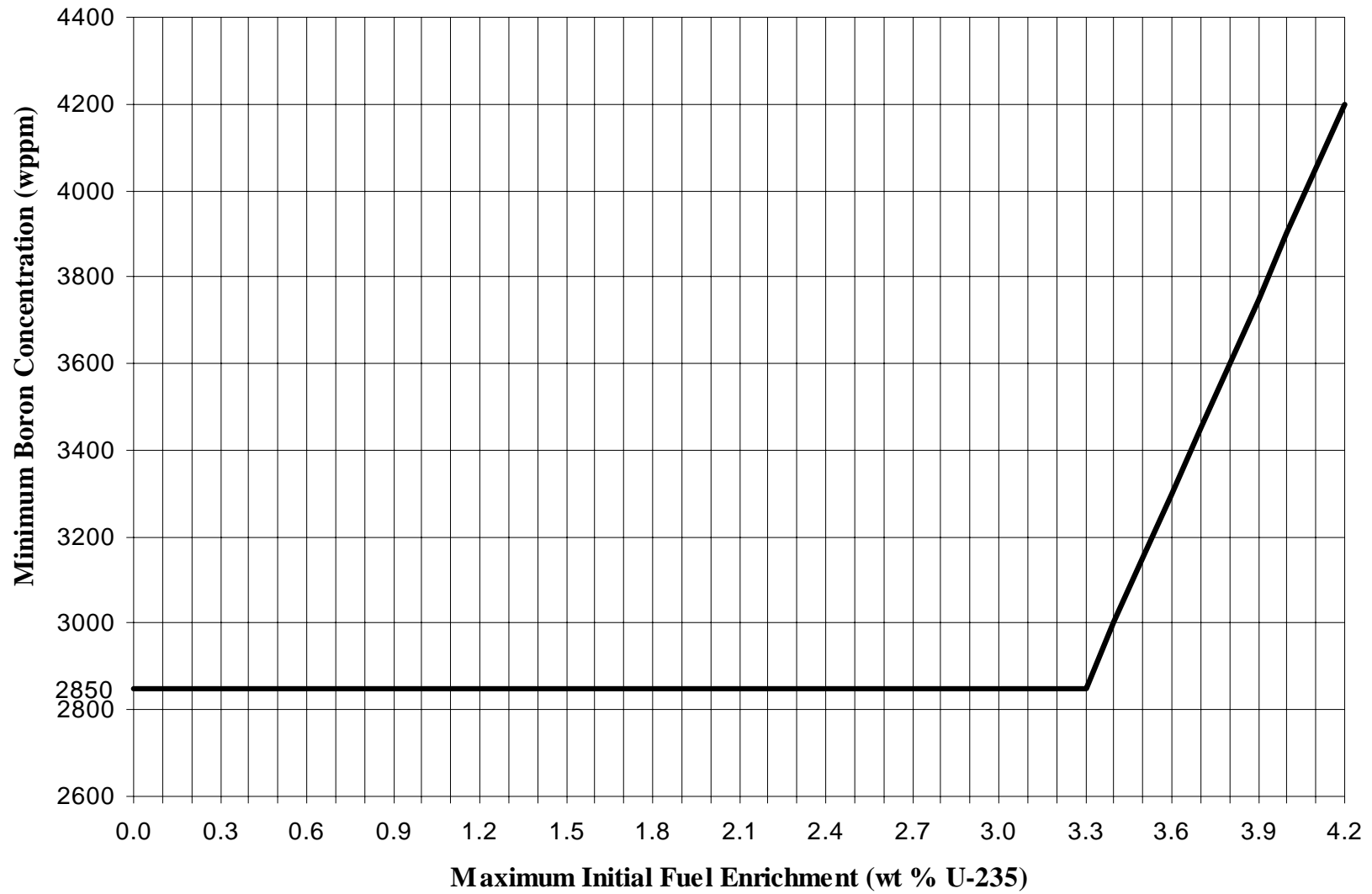
Figure 2 Boron Concentration Curve
