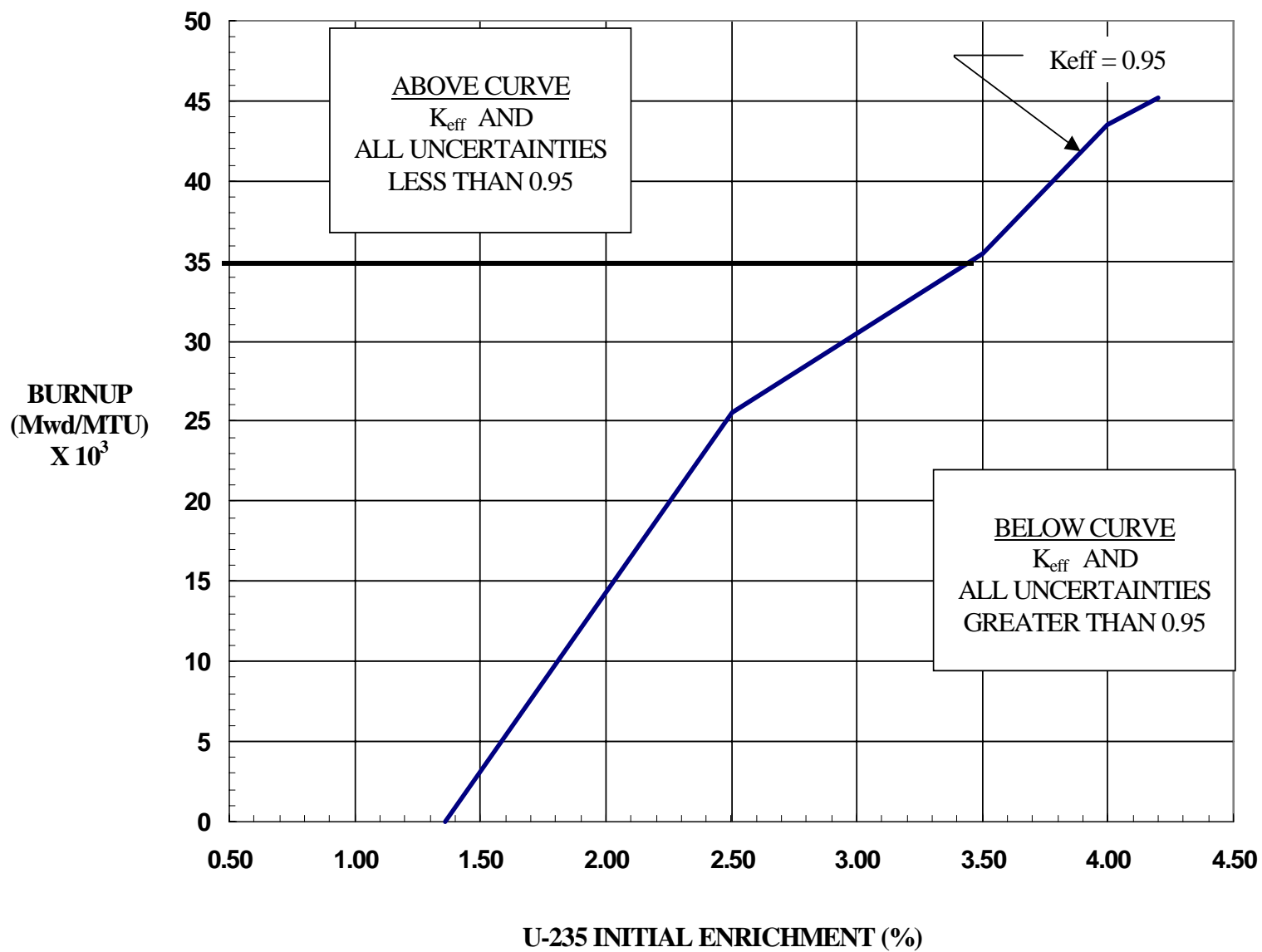
FUEL CRITICALITY ACCEPTABILITY CURVE
