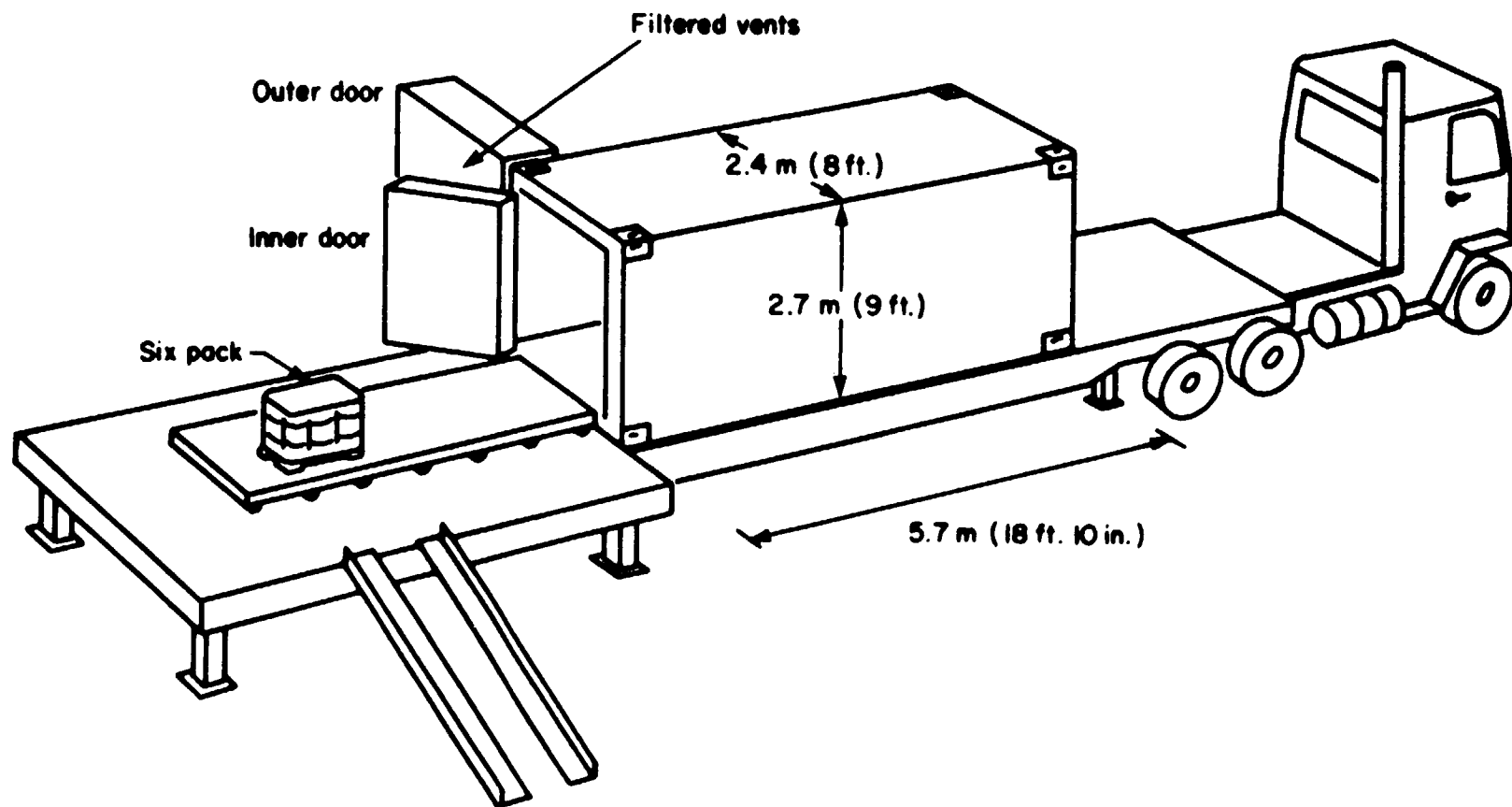
Figure 2. TRUPACT-I transport package.
