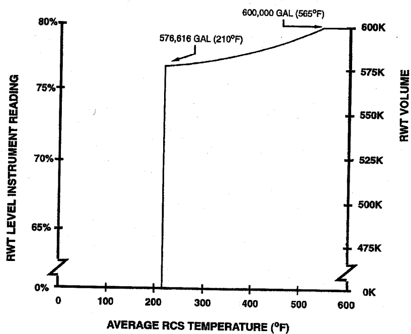
FIGURE 3.5.5-1 Minimum Required RWT Volume
