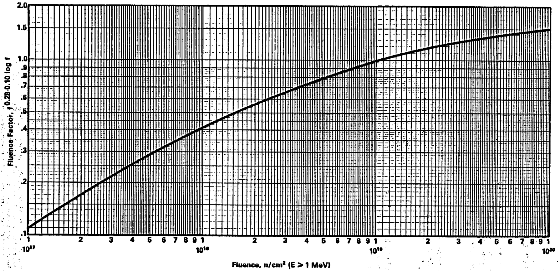
FIGURE 1 Fluence Factor for Use in Equation 2, the Expression for ART NDT
