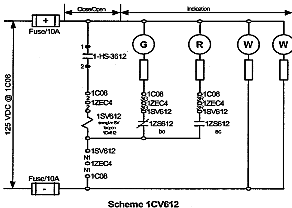
Figure B-1. Solenoid-operated valve control circuit.
