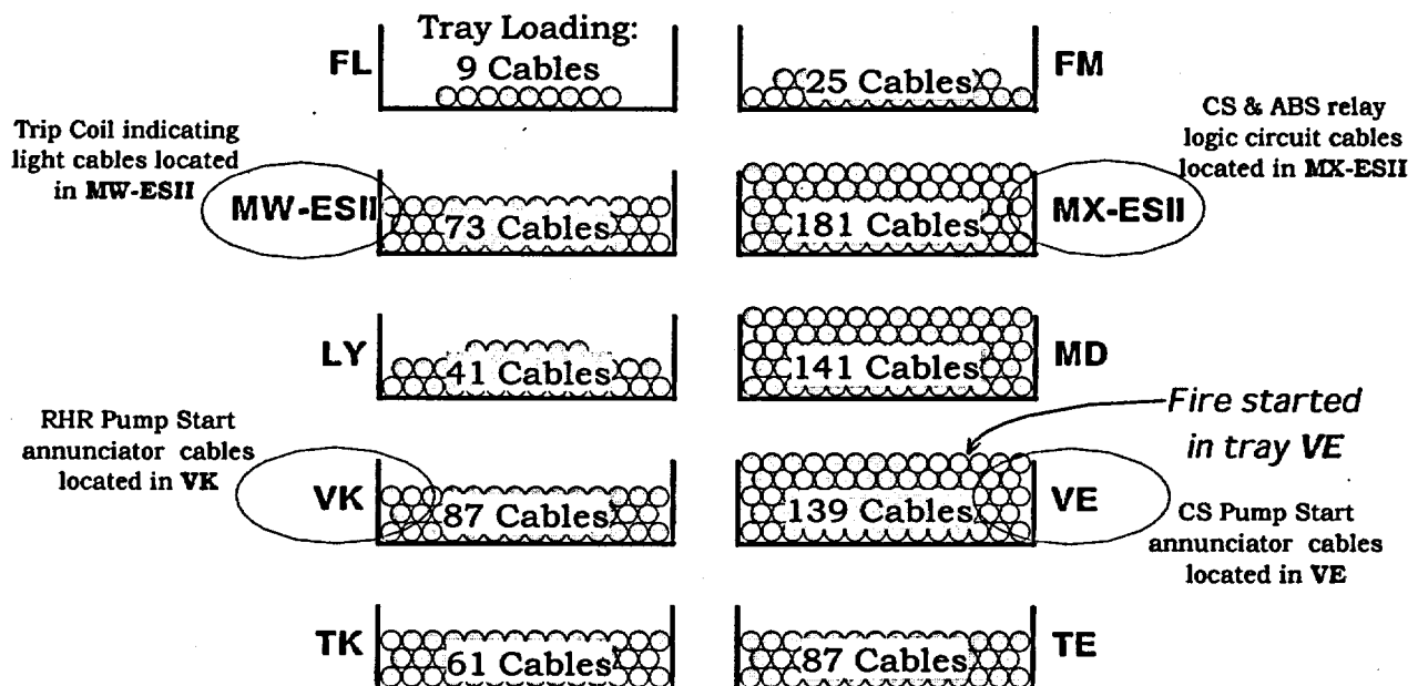
Figure C-9. Cable tray locations and contents. (Ref: Exhibit C1, pp. 30-32 of 69, Physical Damage to Electric Cables and Raceways Involved in the Browns Ferry Nuclear Plant Fire on March 22, 1975 , contained in Regulatory Investigation Report Office of Inspection and Enforcement Region II. )
