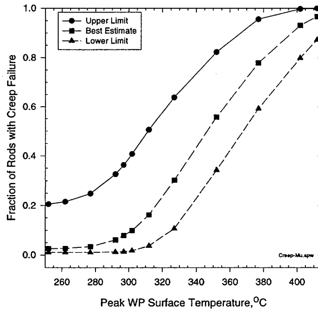
Figure 8. Creep Failure Fraction as a Function of Peak WP Surface Temperature
