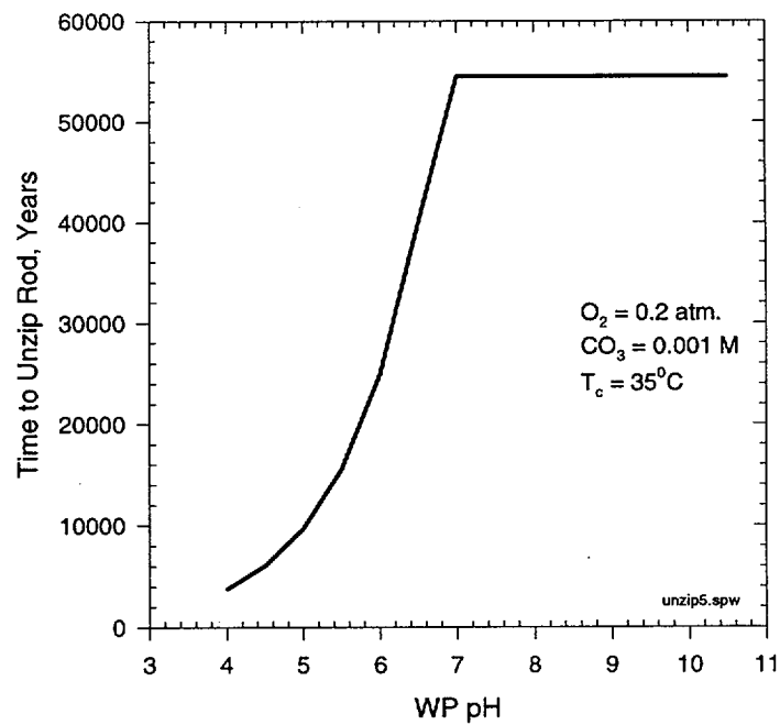
Figure 14. Unzipping Times vs. pH in Waste Package
