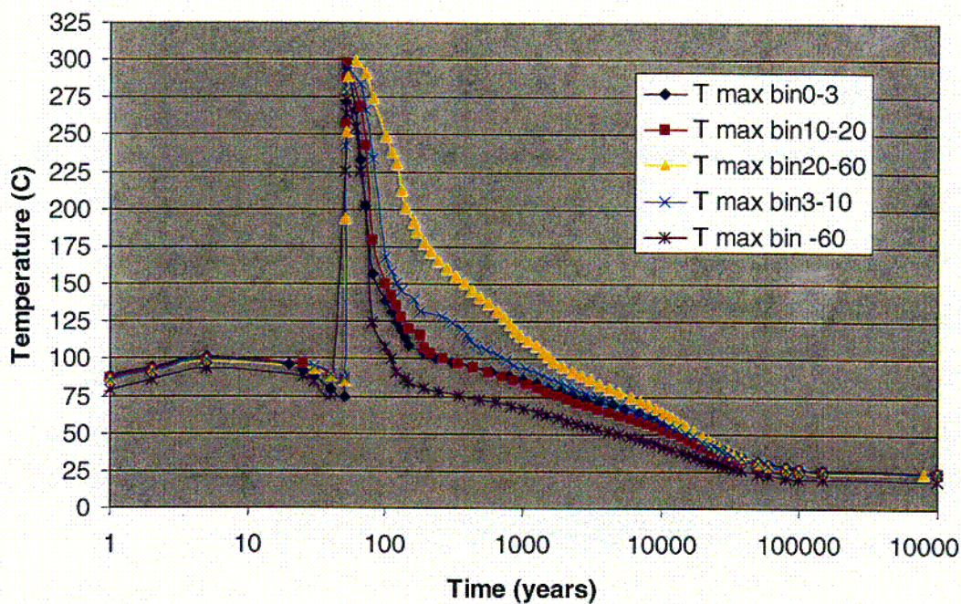
Figure 3. Maximum Temperature Distribution of the 5 Bins of WPs
