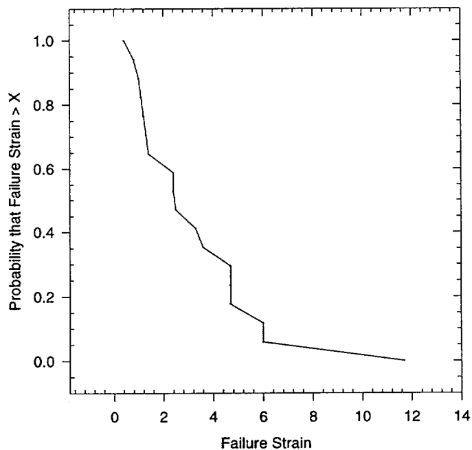
Figure 6. CCDF for Creep Strain Failure Criterion
