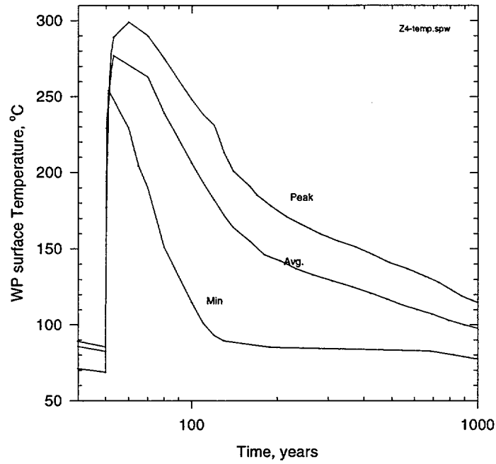
Figure 7. Minimum, Maximum, and Average Temperatures for Bin 4
