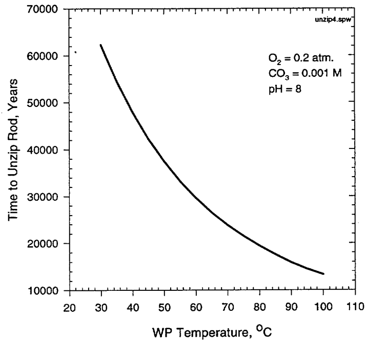
Figure 13. Unzipping Times vs. Temperature in WP
