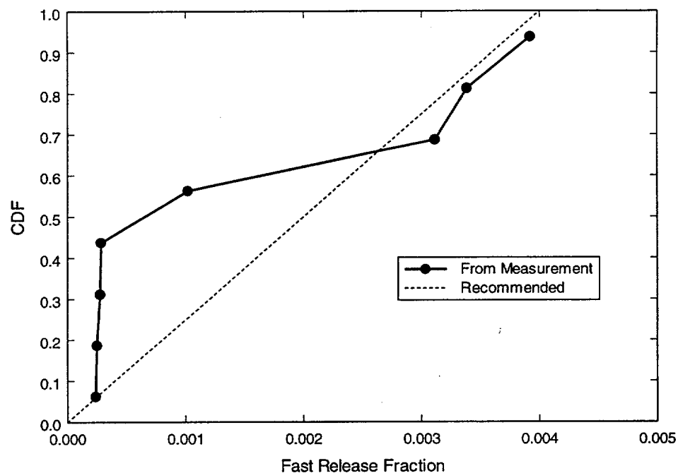
Figure 11. CDF for Fast Radionuclide Release Fraction from Fuel Matrix (DTN: MO00004SPACLD07.043)
