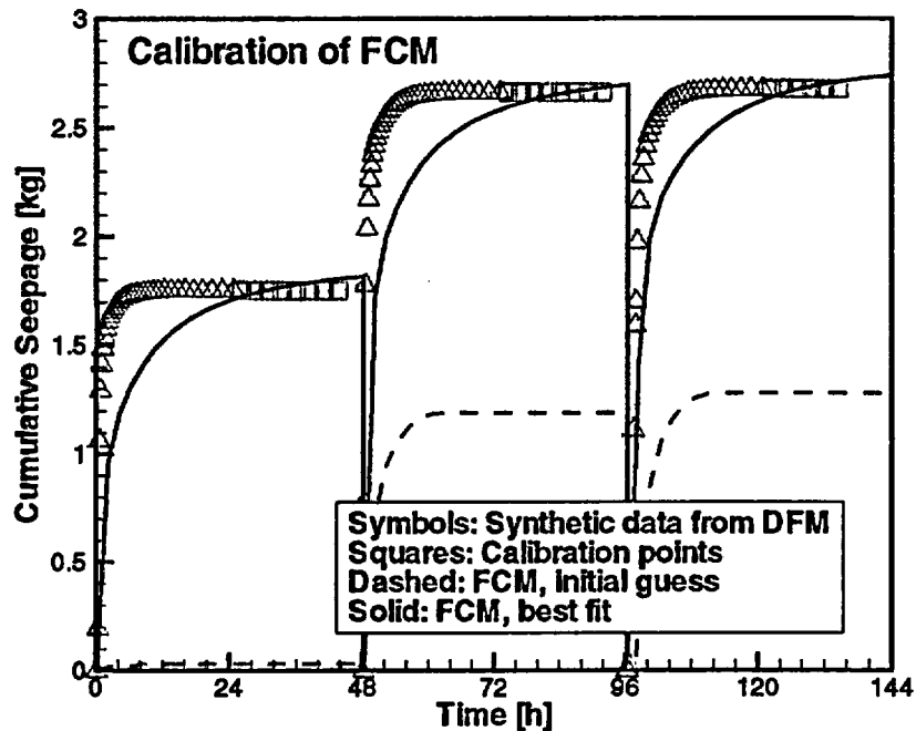
Figure 8. Calibration of FCM Against Late-Time Cumulative-Seepage Data From Three Simulated Liquid-Release Events
