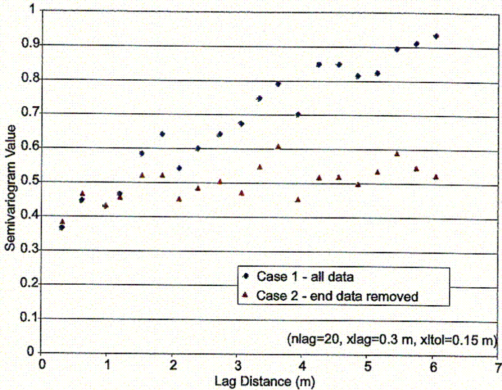
Figure 15. Semivariogram for Post-Excavation Niche 3650 Log-Air-Permeability Values
