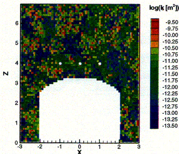
Figure 7. Log-Permeability Field of Fracture Continuum Model
