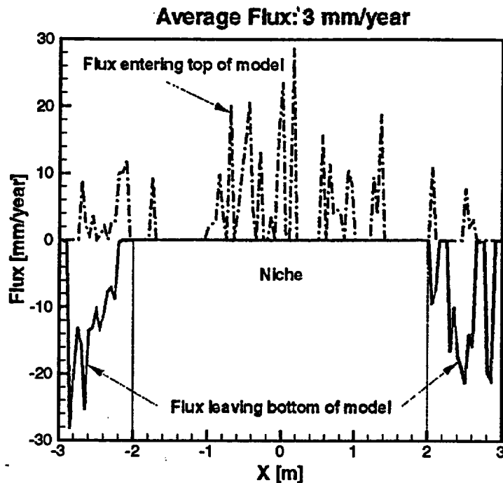
Figure 3. Simulated Steady-State Fluxes Across Top and Bottom of Model Domain, Showing Flow Redistribution as a Result of the Capillary Barrier Effect
