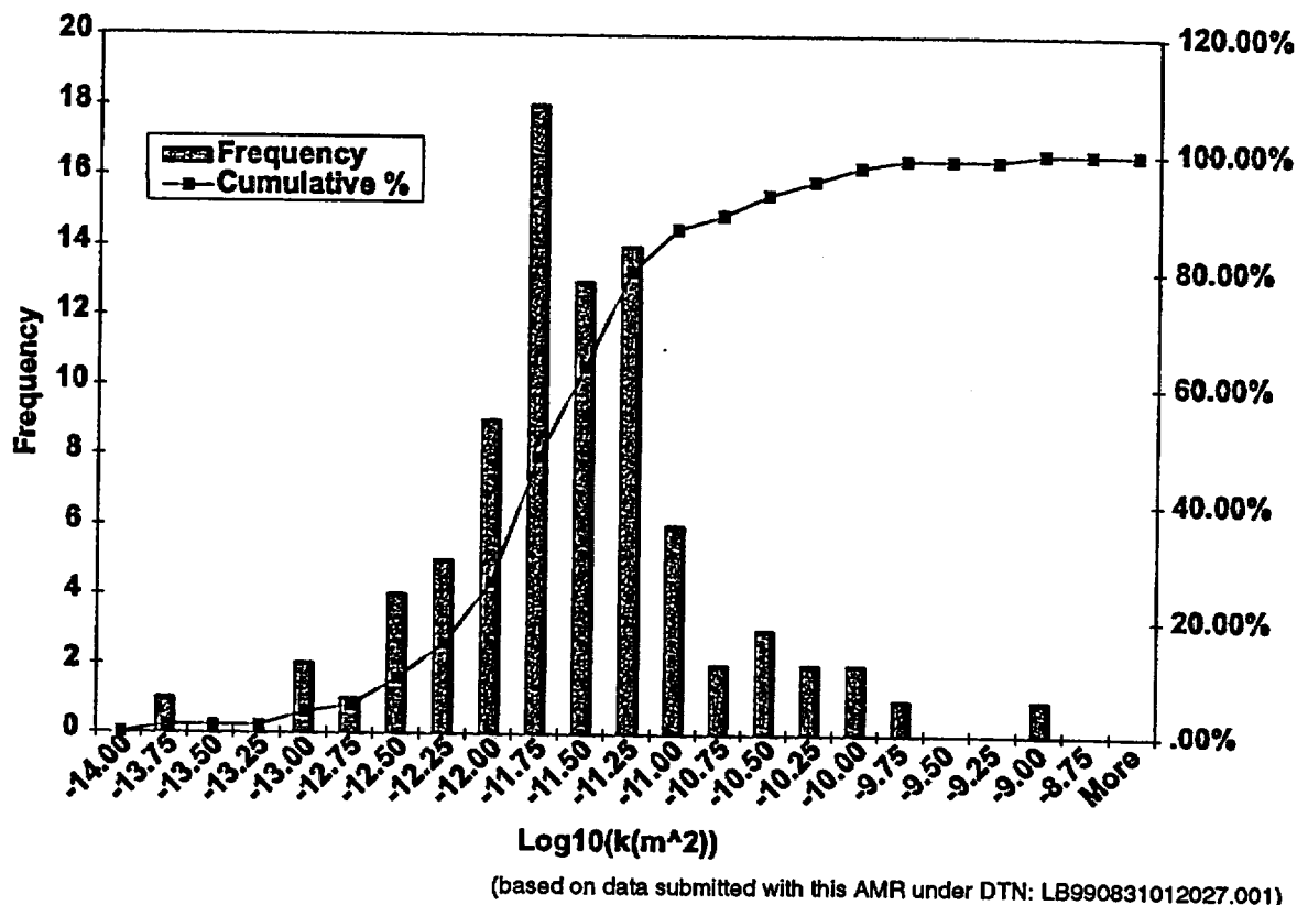
Figure 16. Histogram and Cumulative Distribution Function for Post-Excavation Niche 3650 Log-Air-Permeability Values
