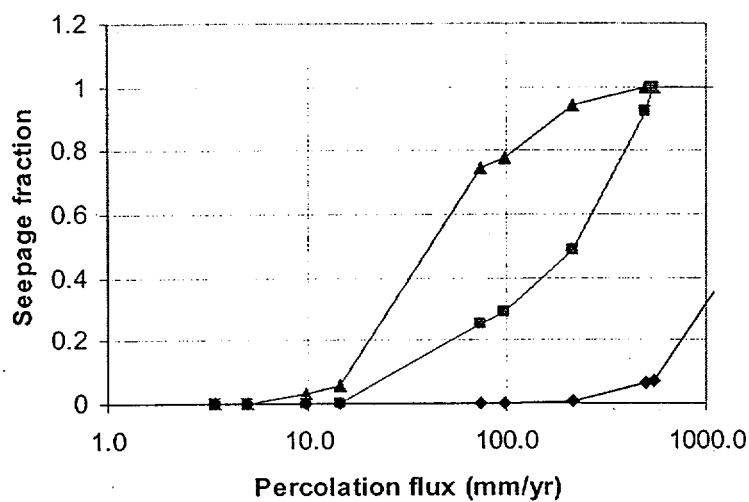
Figure 2. Seepage Fraction vs. Percolation Flux
