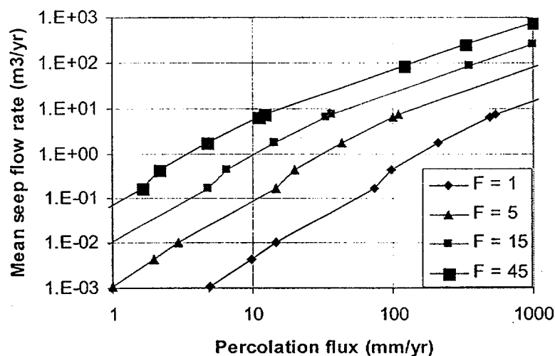
Figure 6. Effect of Flow Focusing on Mean Seep Flow Rate
