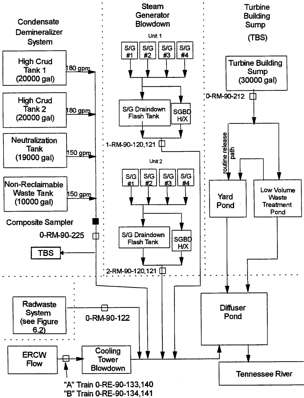
Figure 6.1 LIQUID EFFLUENT RELEASE POINTS
