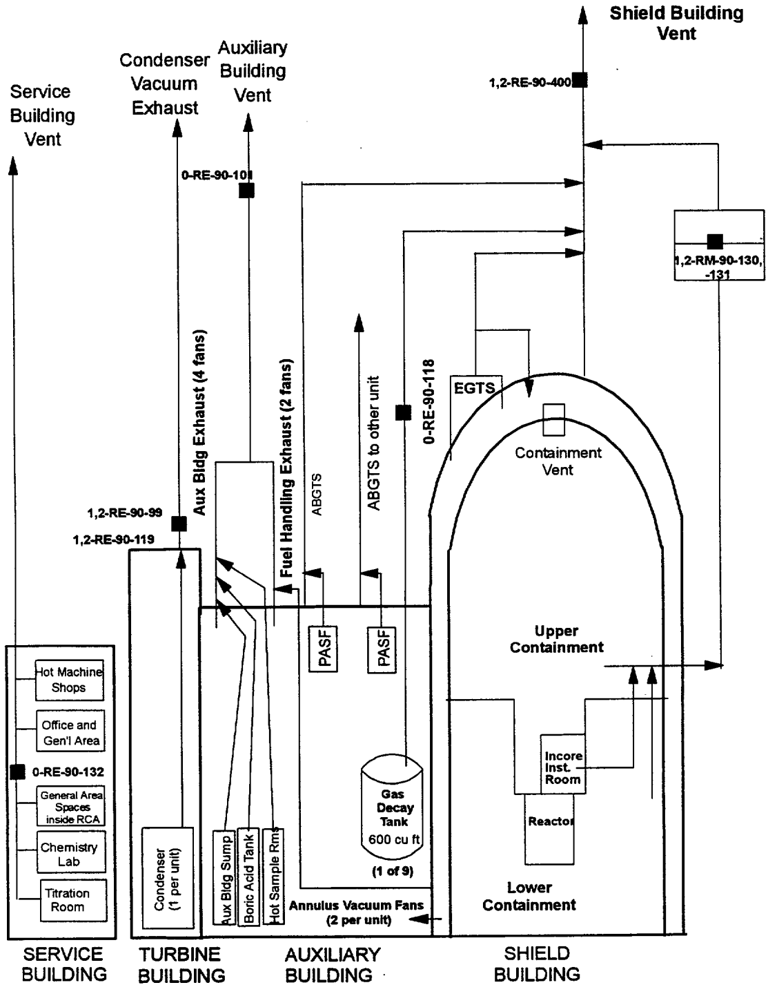
Figure 7.1 GASEOUS EFFLUENT RELEASE POINTS
