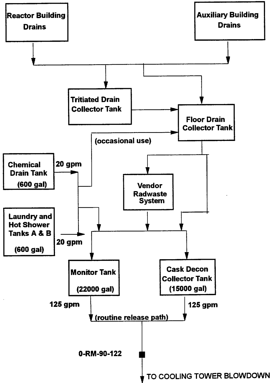
Figure 6.2 LIQUID RADWASTE SYSTEM
