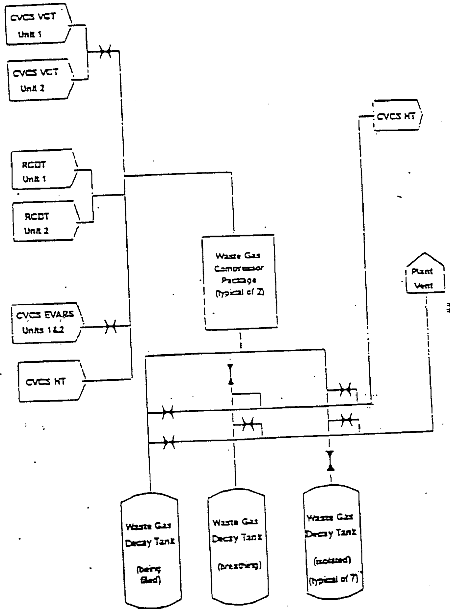
Figure 7.3 GASEOUS RADWASTE TREATMENT SYSTEM (All Vents Are Considered Ground Level)
