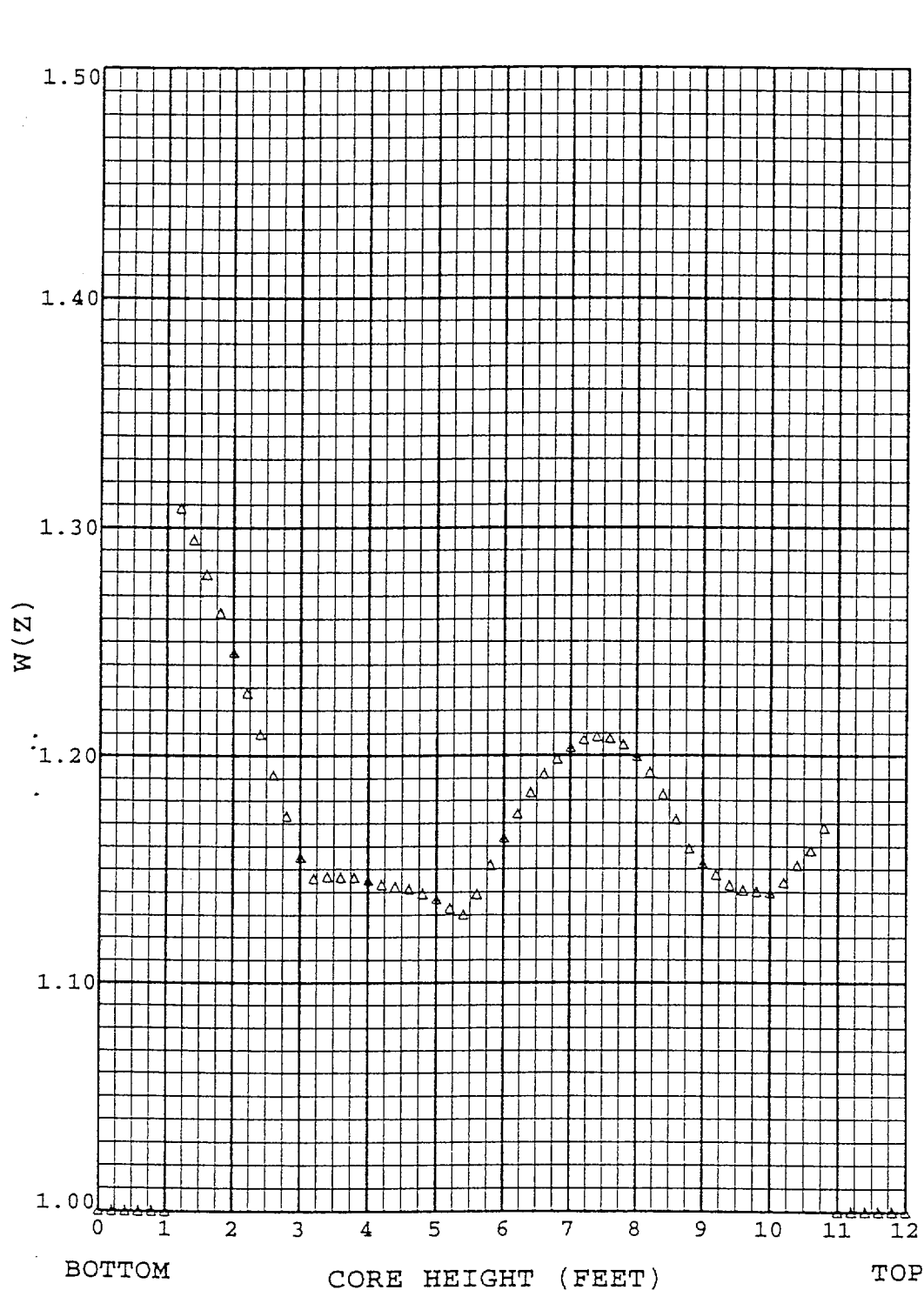
Figure 13 RAOC Summary of Max W(z) at 12000 MWD/MTU With HFP AFD Band of -11/+6 % (Top and Bottom 10% Excluded)
