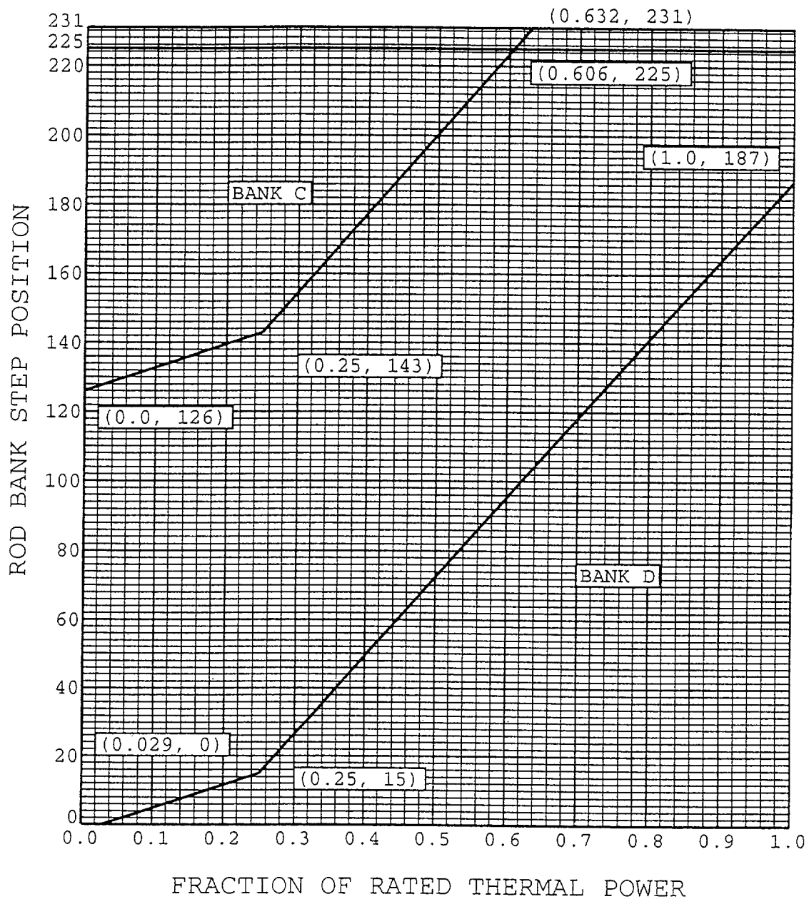
Figure 1 Control Bank Insertion Limits Versus Thermal Power Four Loop Operation For Cycle burnup of 0-4000 MWD/MTU
