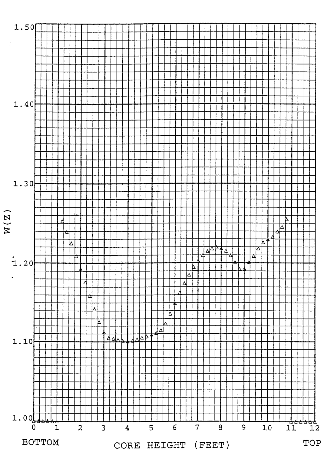
Figure 10 RAOC Summary of Max W(z) at 6000 MWD/MTU With HFP AFD Band of -11/+6 % (Top and Bottom 10% Excluded)
