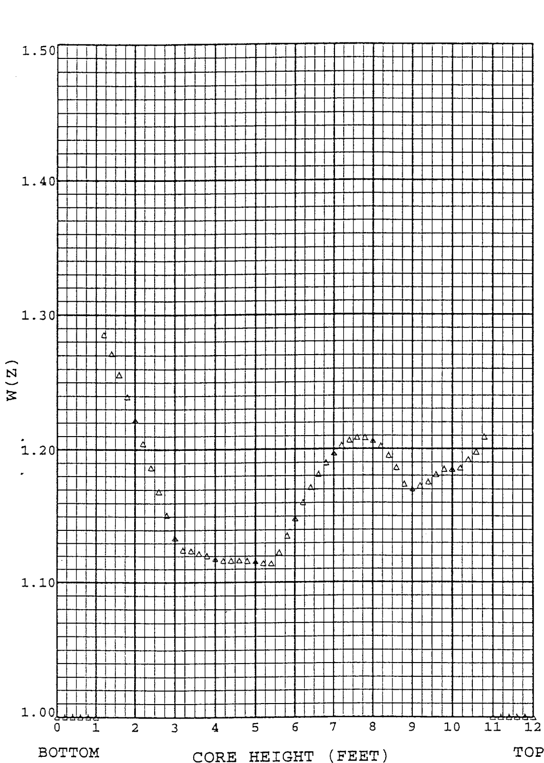
Figure 11 RAOC Summary of Max W(z) at 8000 MWD/MTU With HFP AFD Band of -11/+6 % (Top and Bottom 10% Excluded)
