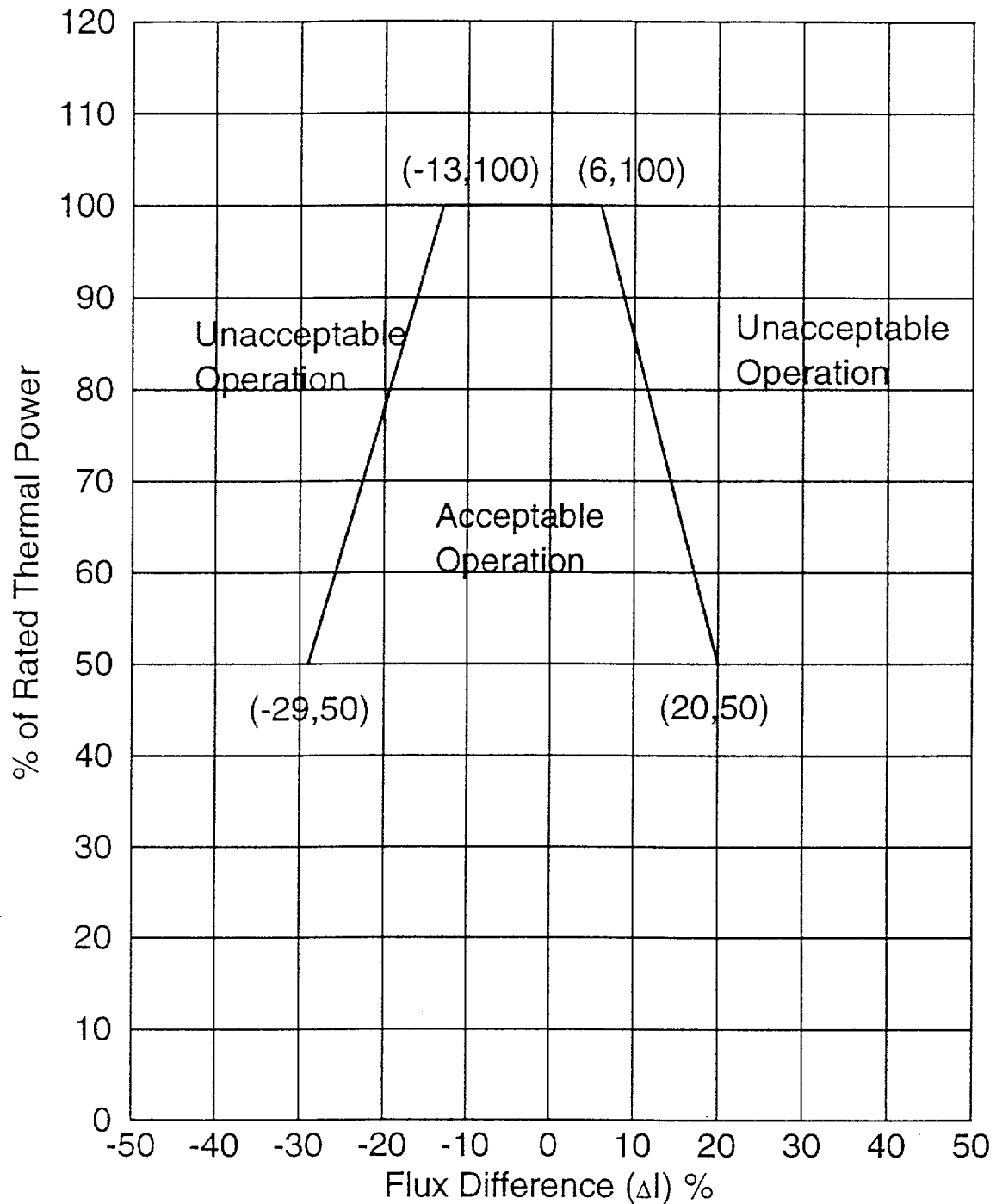
Figure 4 Axial Flux Difference Acceptable Operation Limits as a Function of Rated Thermal Power (RAOC) For Cycle Burnup 0 to 4500 MWD/MTU
