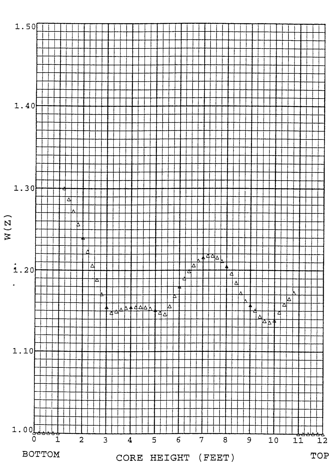
Figure 14 RAOC Summary of Max W(z) at 14000 MWD/MTU With HFP AFD Band of -11/+6 % (Top and Bottom 10% Excluded)
