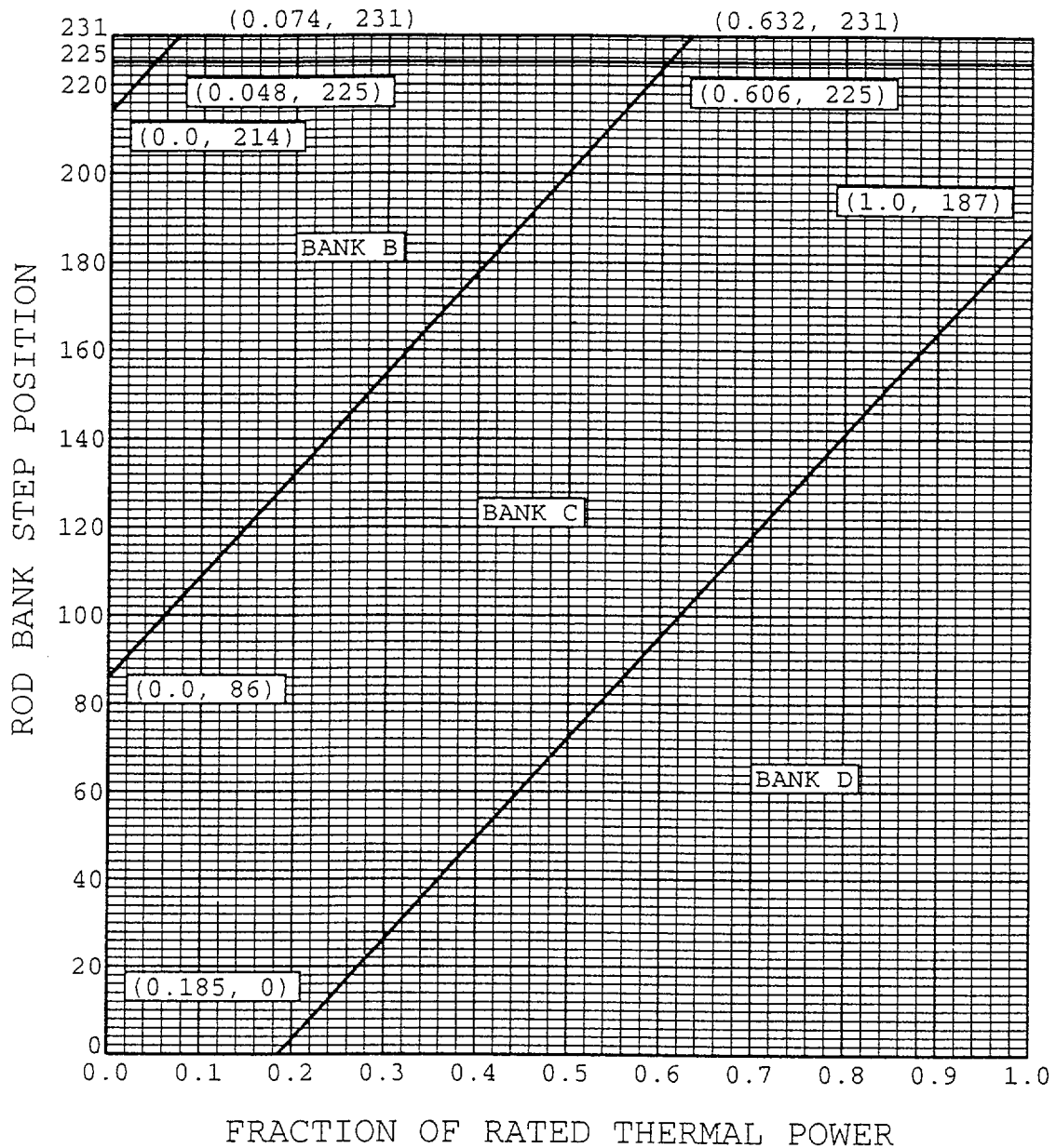
Figure 2 Control Bank Insertion Limits Versus Thermal Power Four Loop Operation For Cycle burnup of 4000-20500 MWD/MTU
