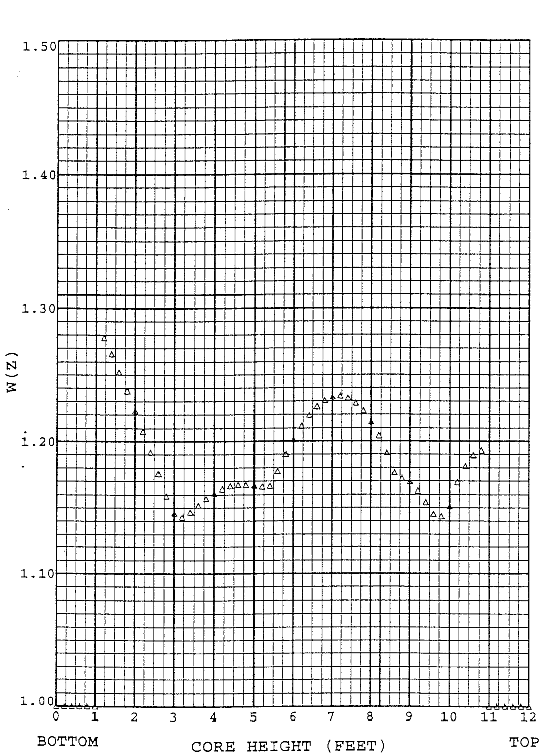
Figure 15 RAOC Summary of Max W(z) at 16000 MWD/MTU With HFP AFD Band of -11/+6 % (Top and Bottom 10% Excluded)
