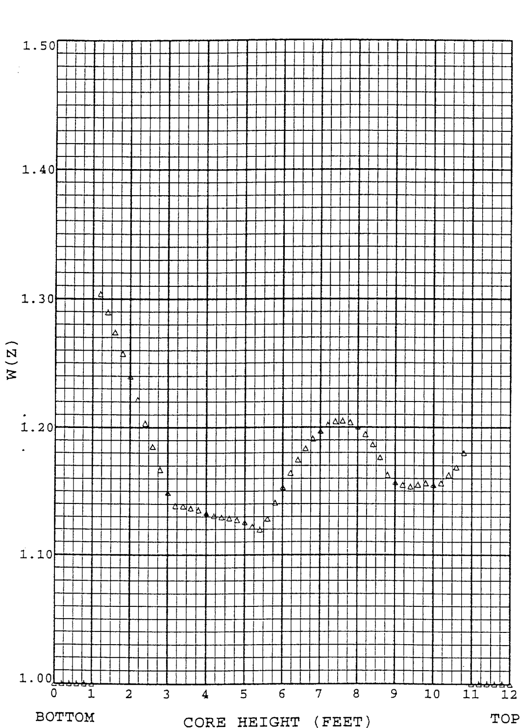
Figure 12 RAOC Summary of Max W(z) at 10000 MWD/MTU With HFP AFD Band of -11/+6 % (Top and Bottom 10% Excluded)
