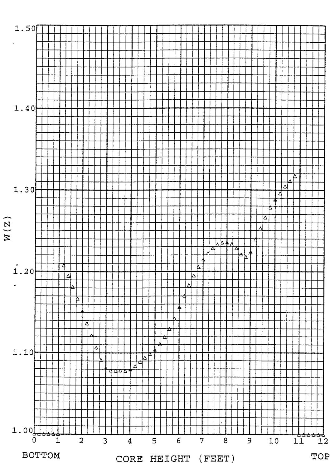
Figure 9 RAOC Summary of Max W(z) at 4000 MWD/MTU With HFP AFD Band of -11/+6 % (Top and Bottom 10% Excluded)
