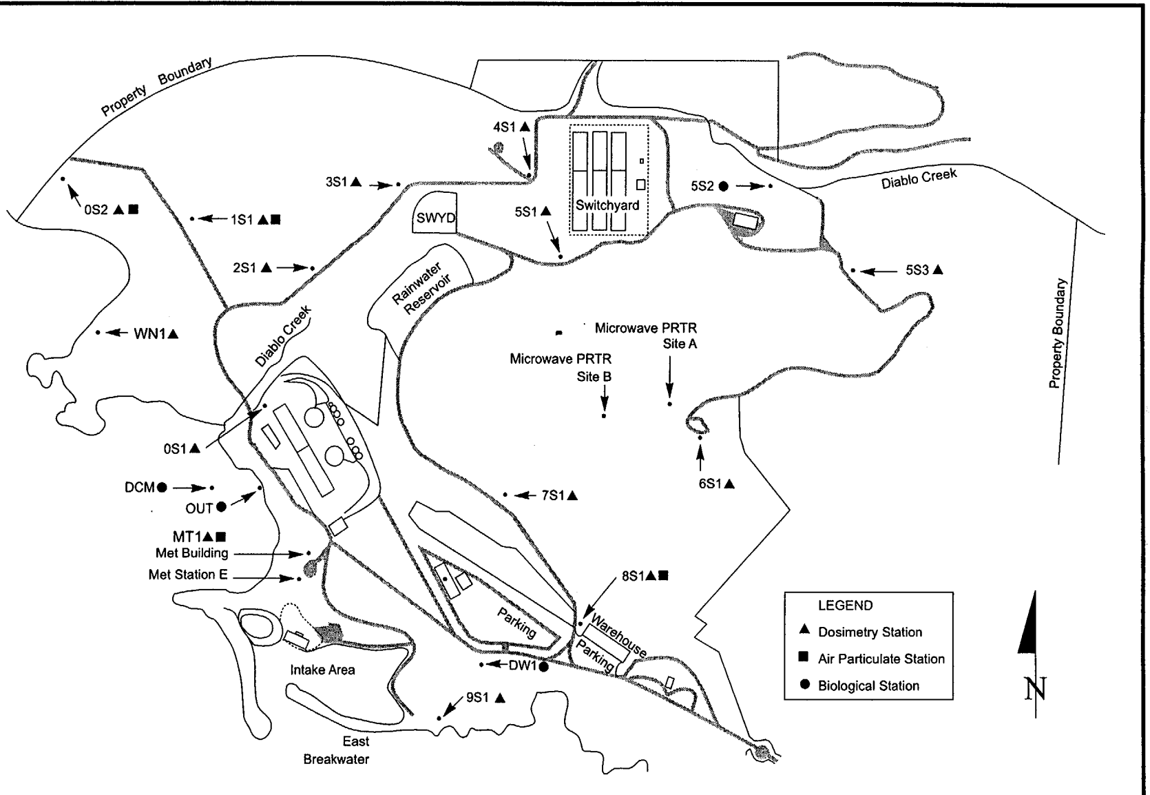
Figure 2. Units 1 and 2 Diablo Canyon on-site stations.
