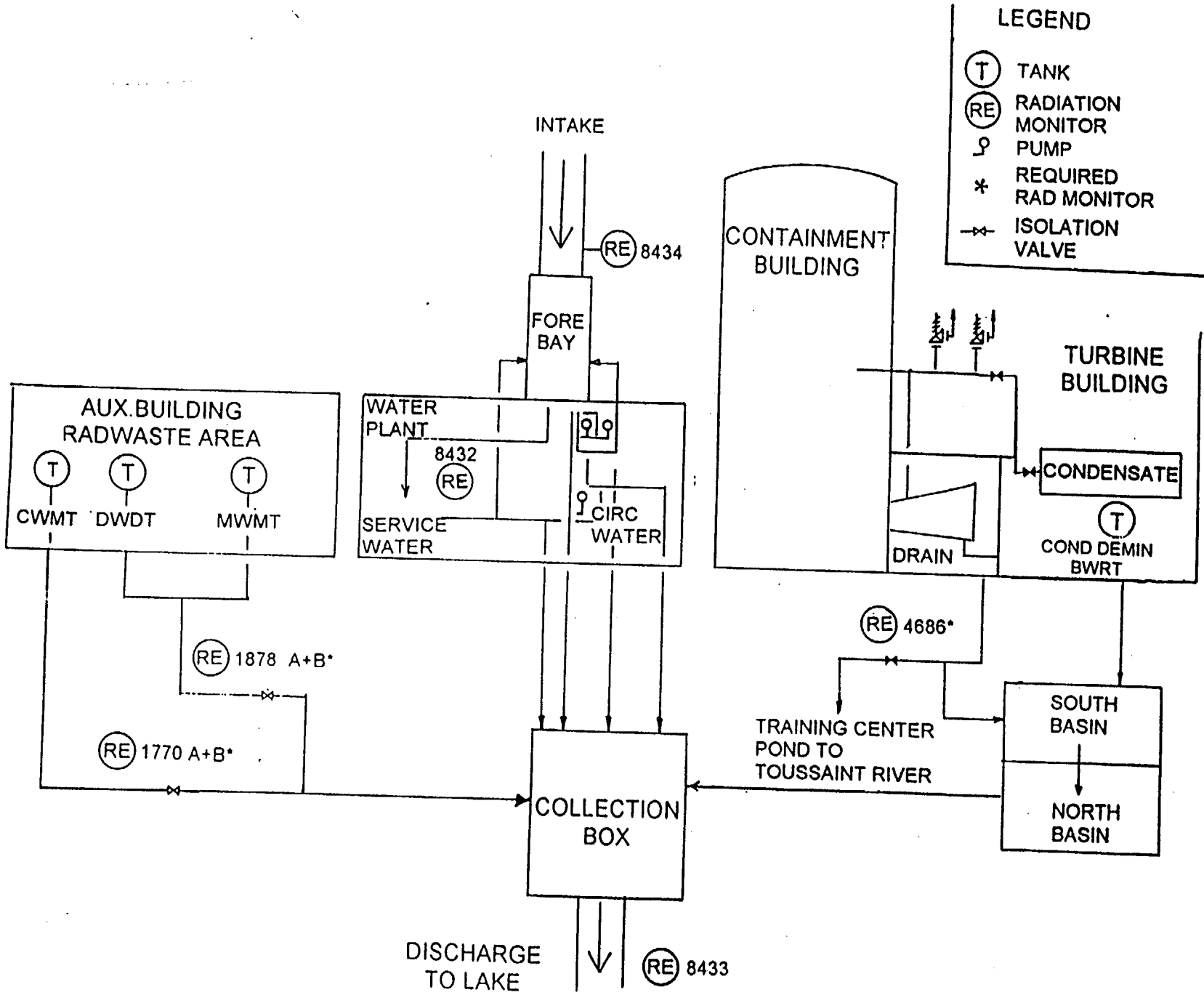
Liquid Radioactive Effluent Monitoring and Processing Diagram
