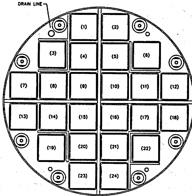
BWR Basket Fuel Loading Positions
