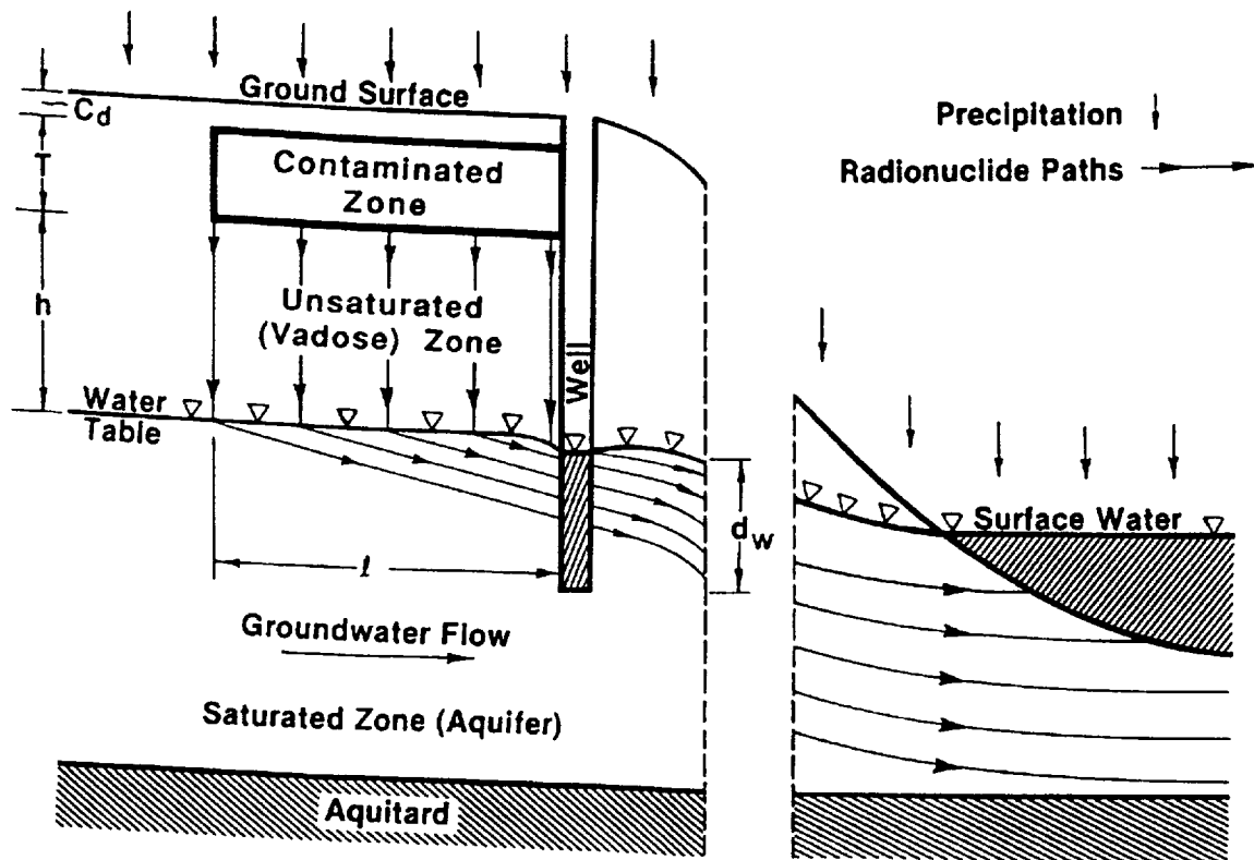
Figure 2-7. RESRAD conceptual representation of the subsurface transport pathways (from Yu et al., 1993a)
