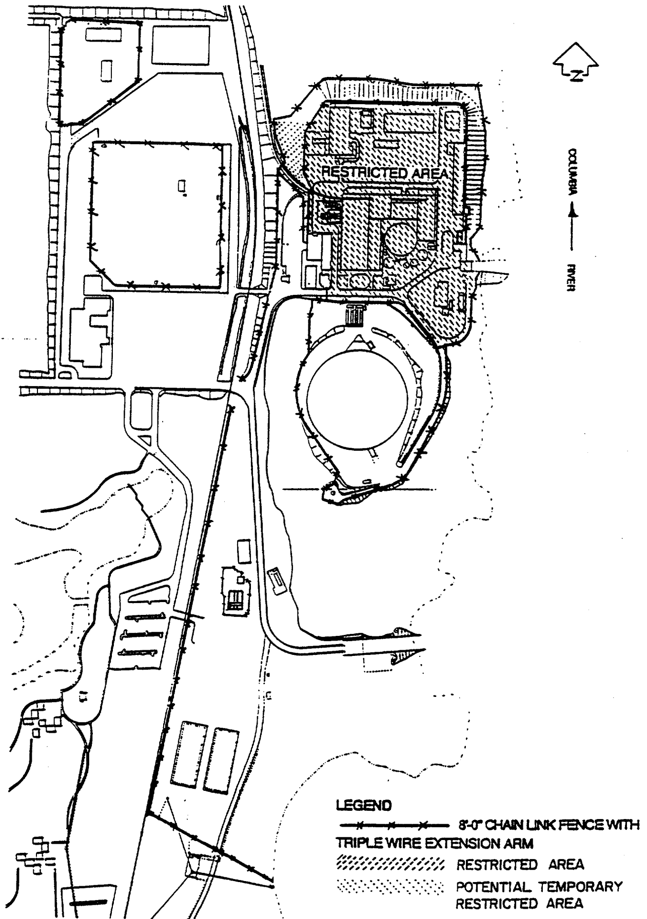
Trojan Plant Fence Layout Figure 1.1-3
