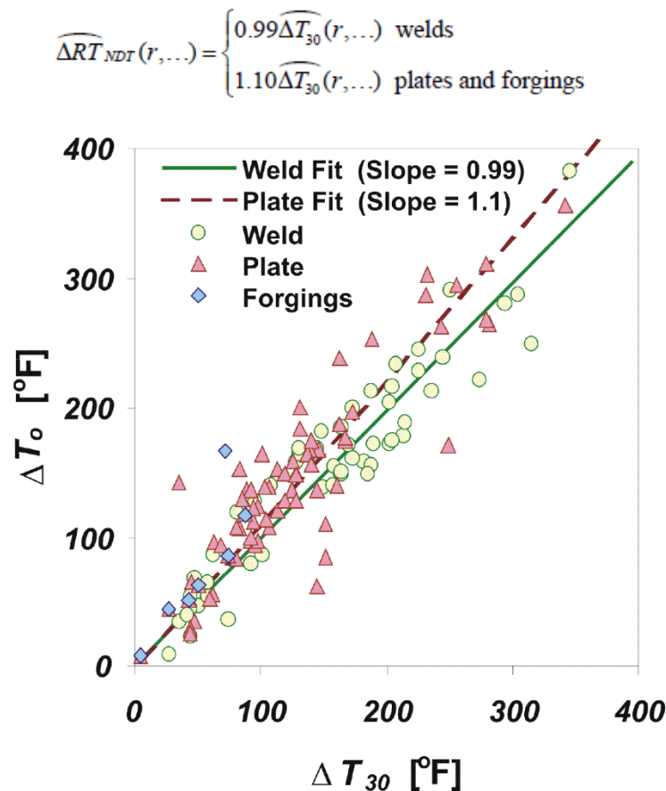
Figure 14: Relationship between the change in the fracture-toughness index temperature ( \Delta T_0 \approx \Delta RT_{NDT} ) change in the 30 ft-lbf CVN transition temperature ( \Delta T_{30} ) for welds and plates/forgings produced by irradiation. The difference in the best-fit slopes is statistically significant (from [16]).
