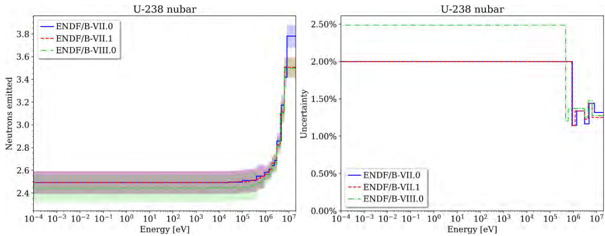
Figure 2-25 238 U Fission Neutron Multiplicity Nominal Data and Uncertainty
