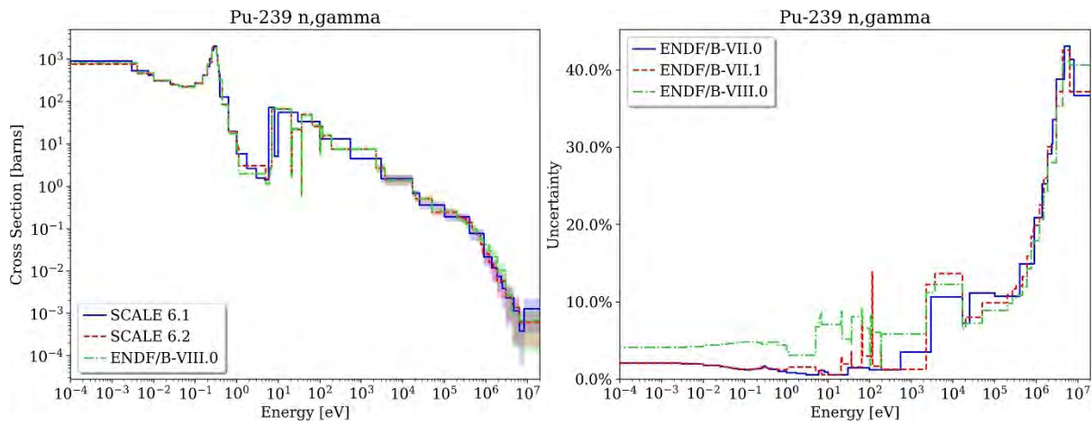
Figure 2-24 239 Pu (n, \gamma ) Nominal Data and Uncertainty
