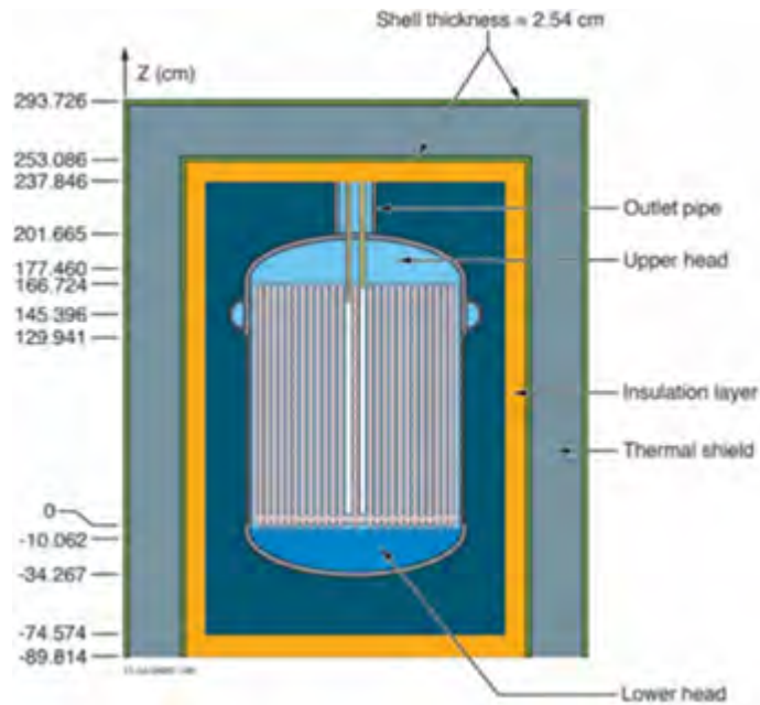
Figure 4-7 Vertical Cross Section of the MSRE Benchmark (Shen et al., 2019) 2
