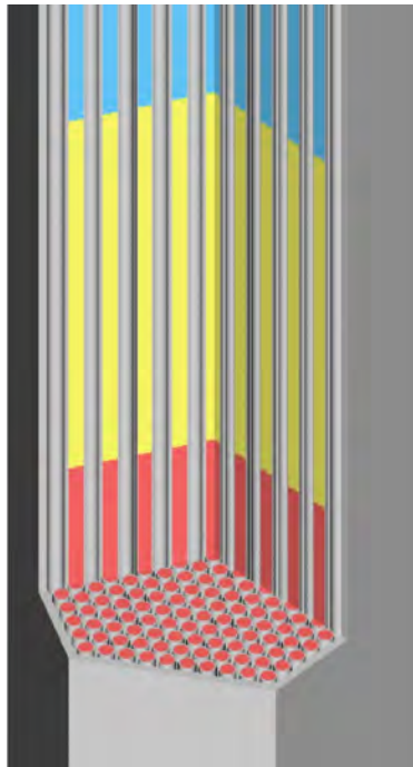
Figure 5-45 ABR-1000: SCALE Fuel Assembly Model 46
