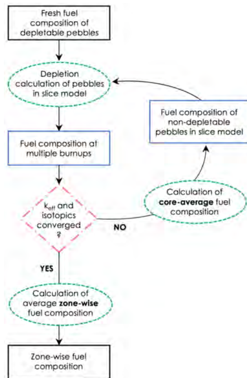
Figure A-1 PB-FHR-Mk1: Flowchart Showing the Process to Determine Fuel Compositions in the Individual Axial Fuel Zones
