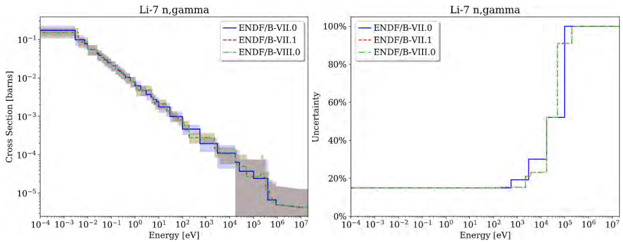
Figure 2-33 {}^7\text{Li} (n, \gamma ) Nominal Data and Uncertainty
