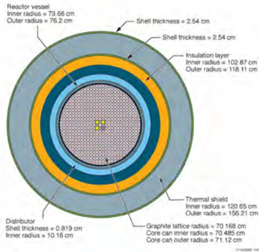
Figure 4-6 Horizontal Cross Section of the MSRE Benchmark (Shen et al., 2019) 1
