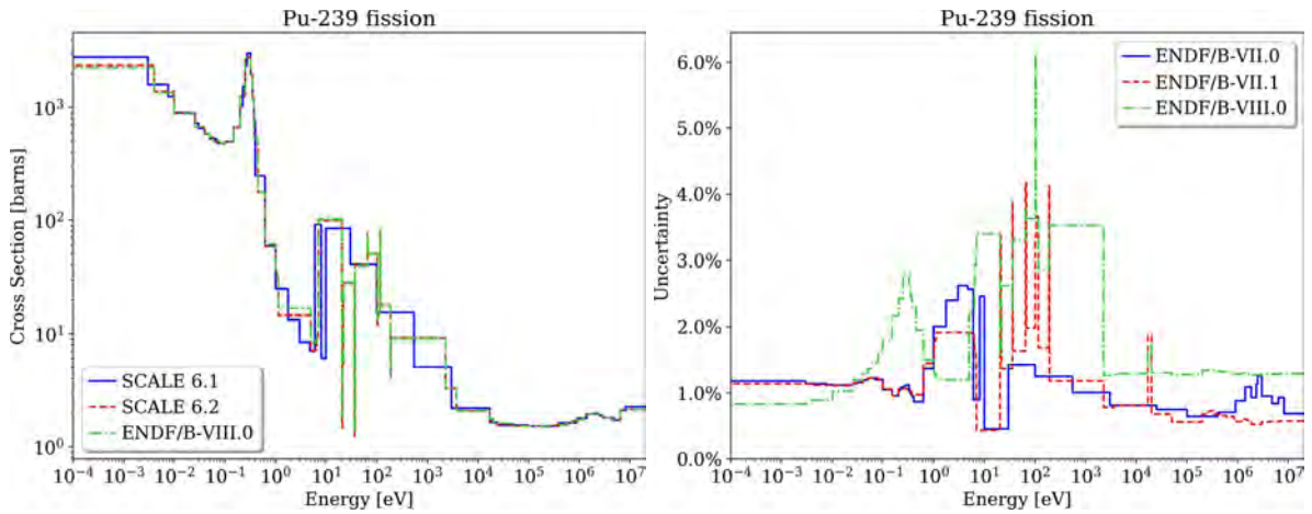
Figure 2-23 239 Pu Fission Nominal Data and Uncertainty
