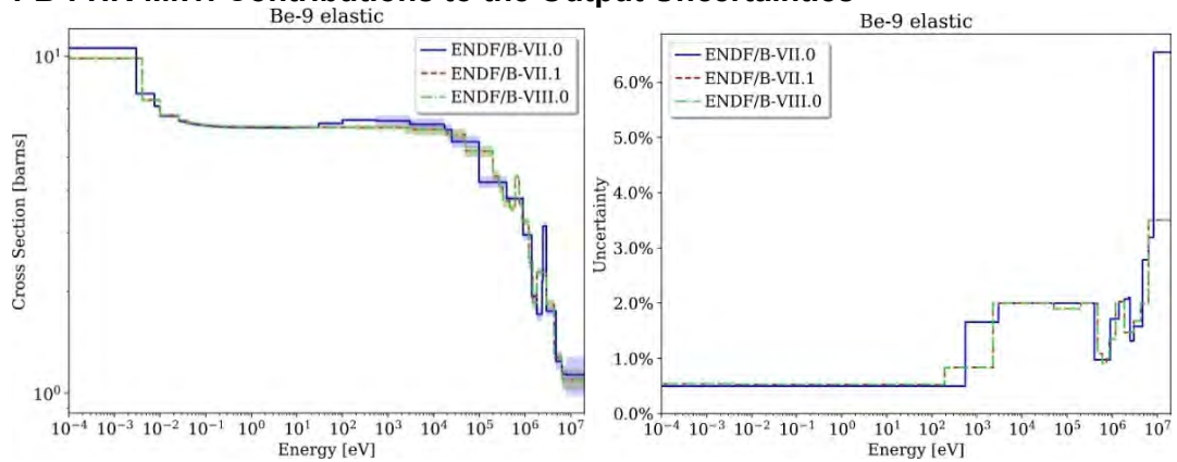
Figure 5-11 ^9\text{Be} Elastic Scattering Nominal Data and Uncertainty
