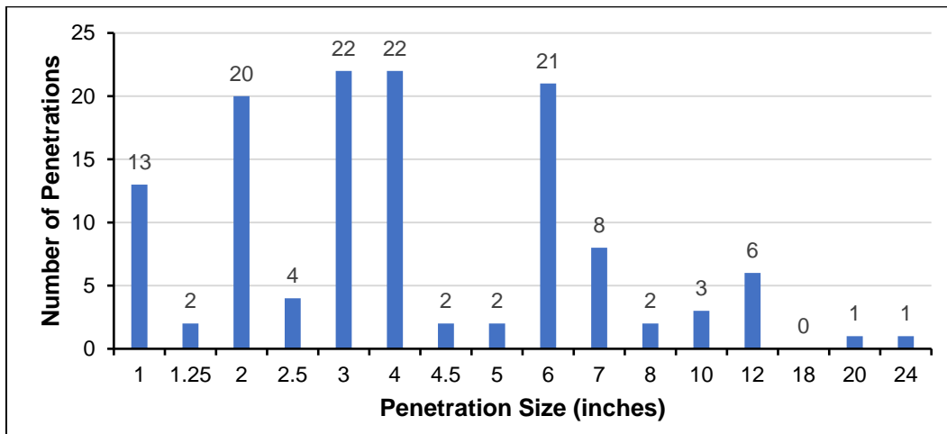
Figure 2-2 Sleeve/Core-Bored Penetration Internal Diameters
