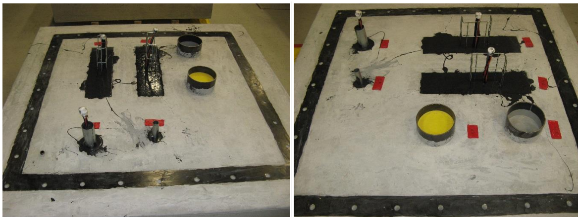
Figure 4-18 Photos of Test Deck 4 After Seal Assembly Installation
