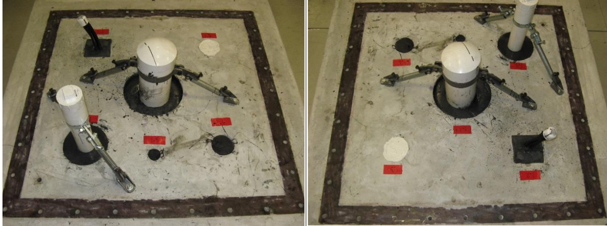
Figure 4-10 Photos of Test Deck 1 After Seal Assembly Installation
