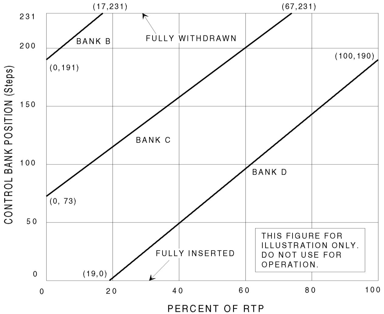
Figure B 3.1.6 (page 1 of 1) Control Bank Insertion vs. Percent RTP
