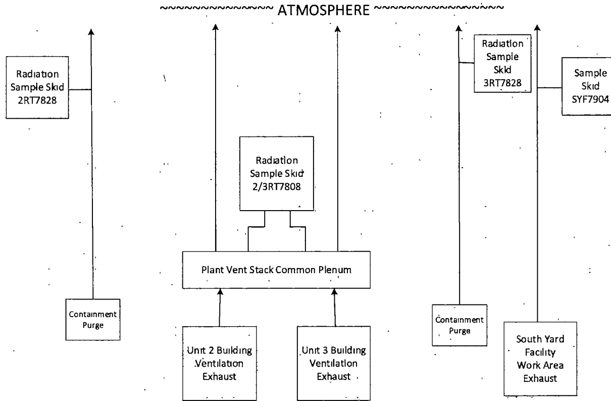
Figure 4-6 SONGS Radioactive Gaseous Waste Treatment Systems
