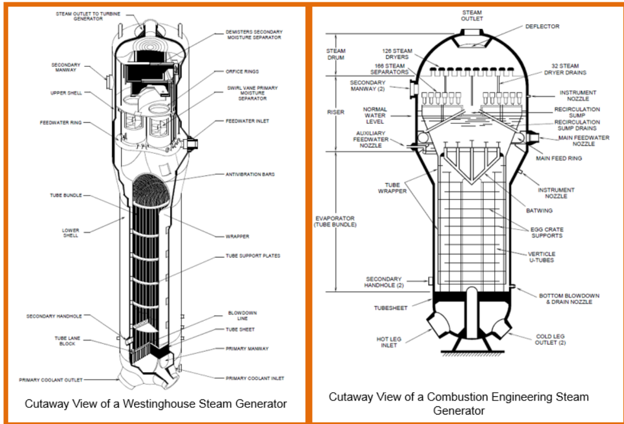
Figure 3-18 Cutaway views of Westinghouse and Combustion Engineering U-tube steam generators
