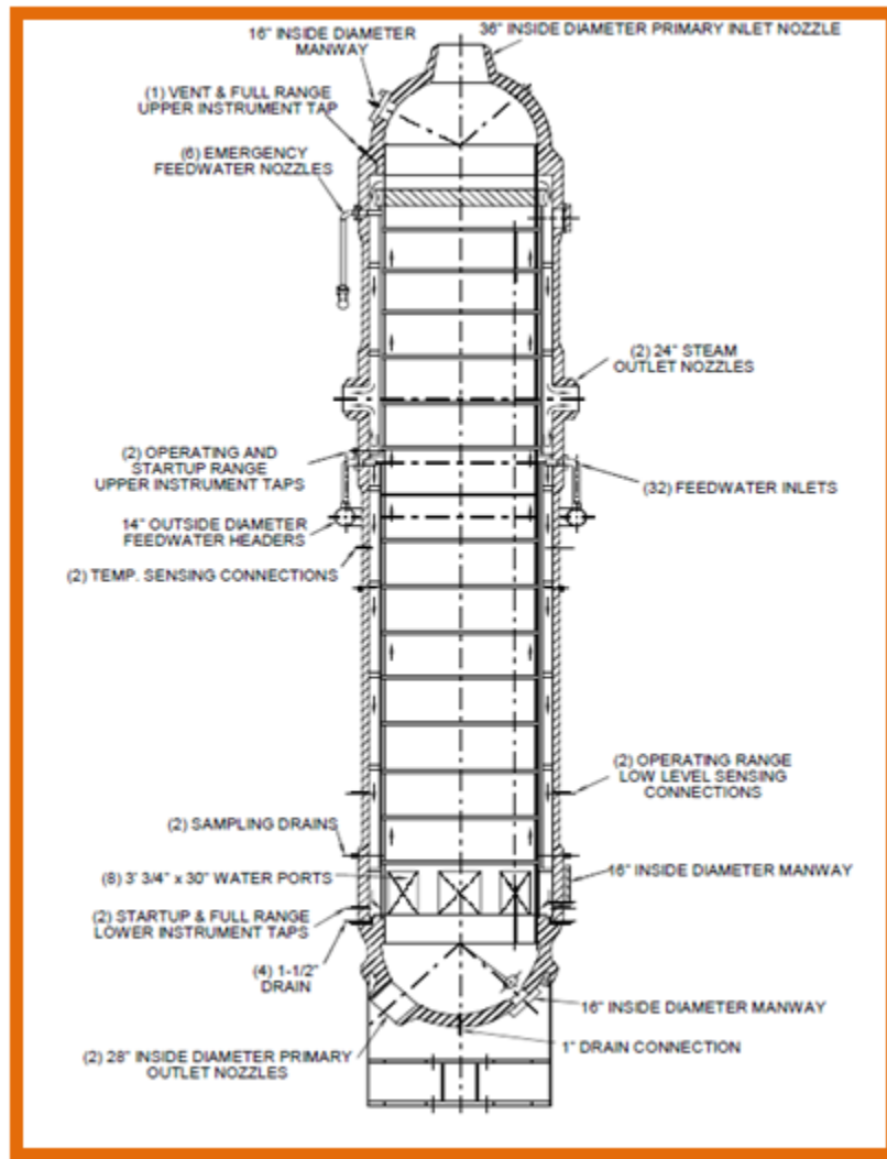
Figure 3-19 Cutaway view of Babcock and Wilcox once-through steam generator
