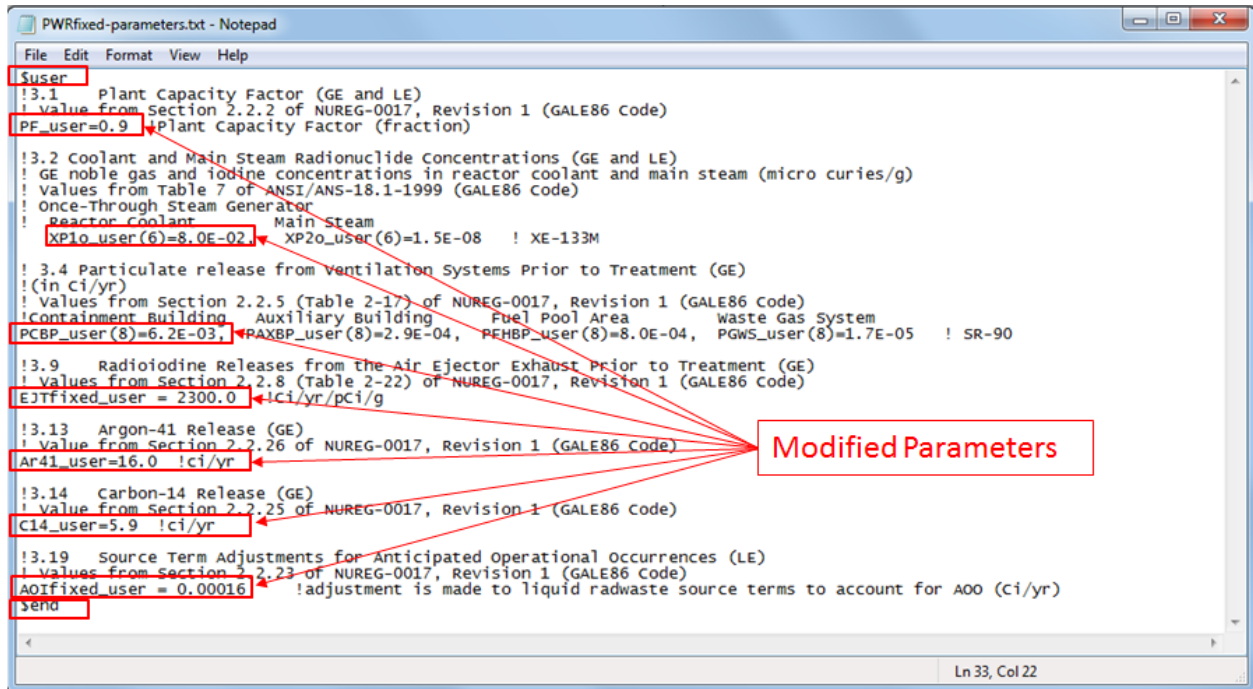
Figure 4-7 Example of a modified PWRfixed-parameters.txt file
