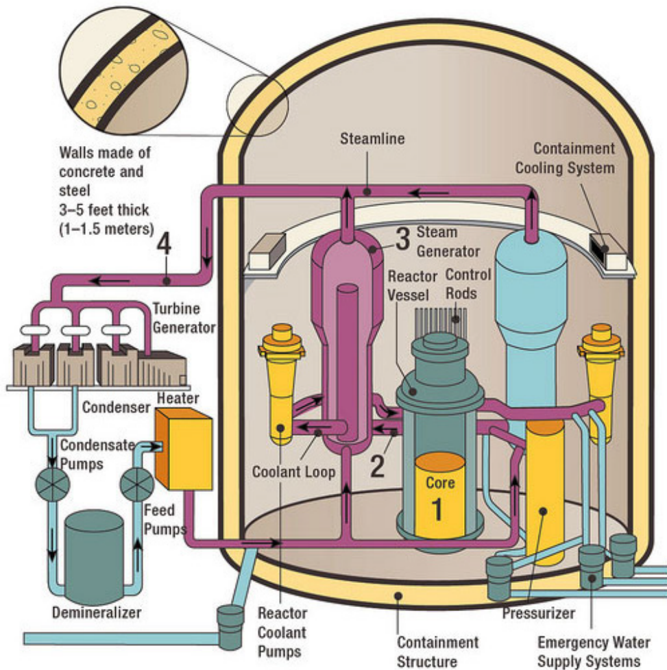
Figure 3-9 Basic structure of a PWR
