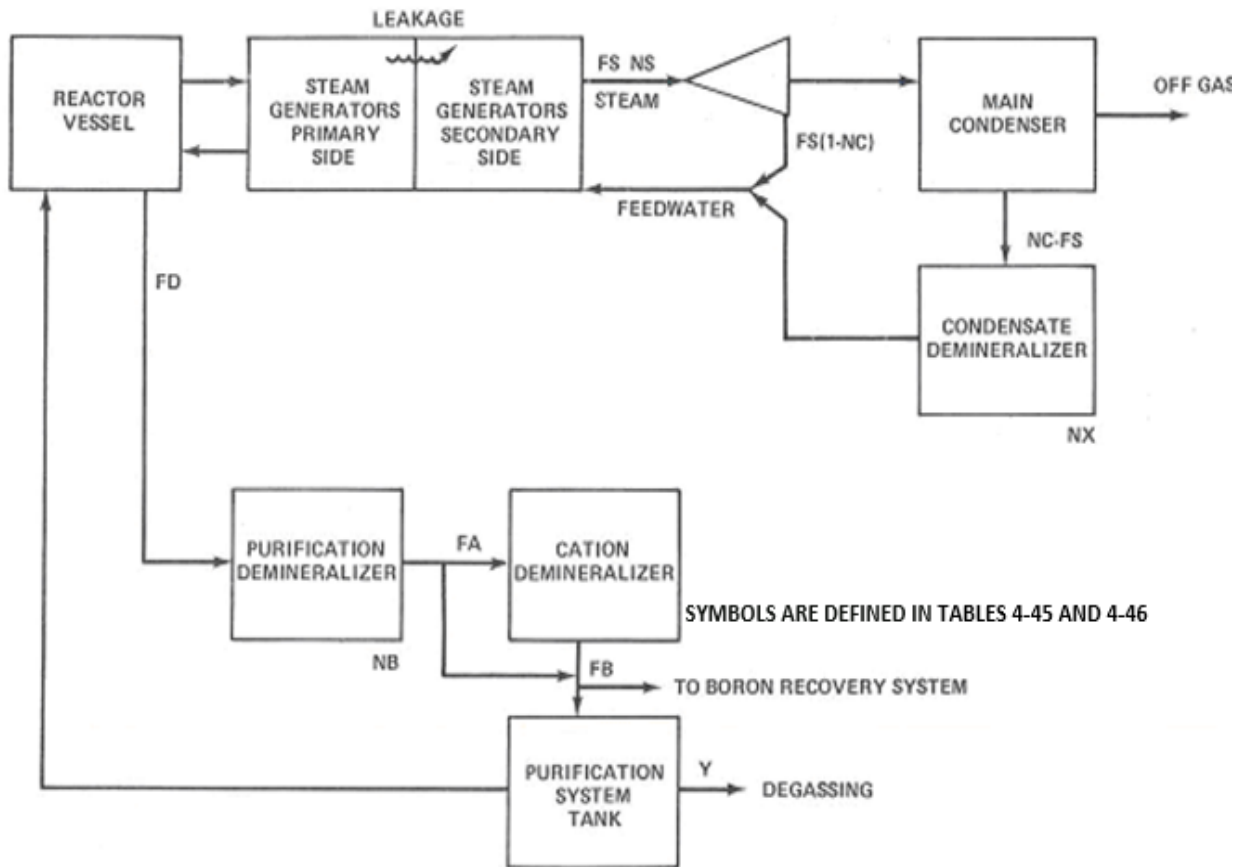
Figure 4-5 Removal paths for the reference PWR with once-through steam generators
