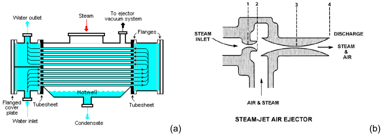
Figure 3-61 Diagram of turbine condenser (a) and steam-jet air ejector (b)
