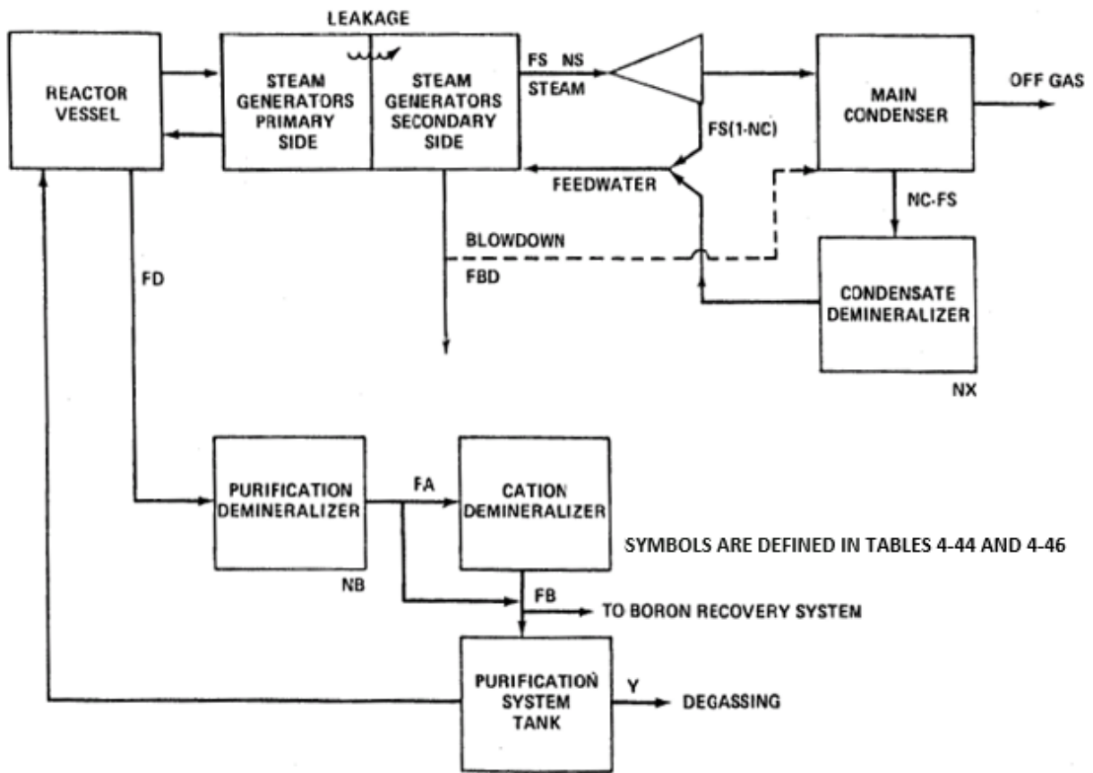
Figure 4-4 Removal paths for the reference PWR with U-tube generators
