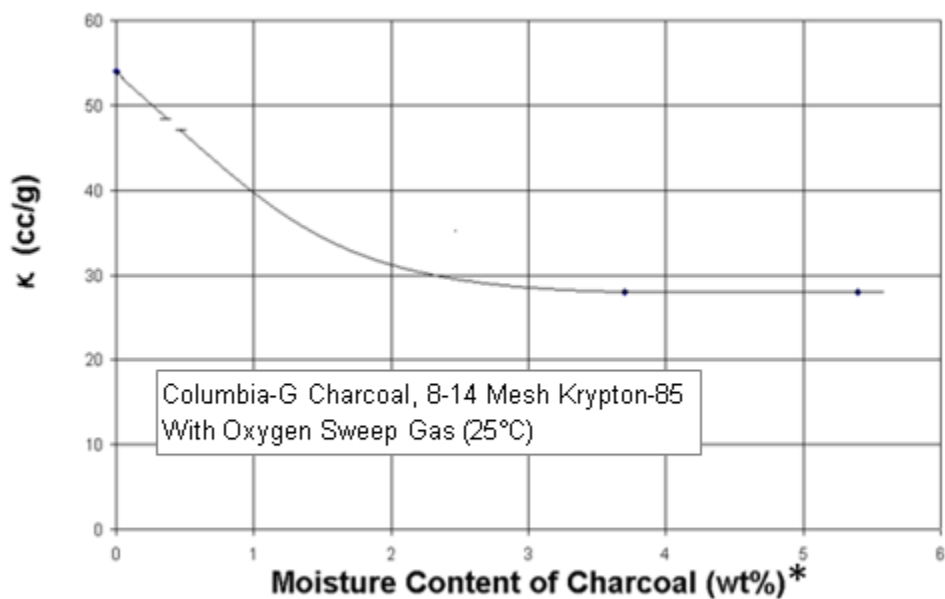
Figure 4-2 Effect of moisture content on the dynamic adsorption coefficient
