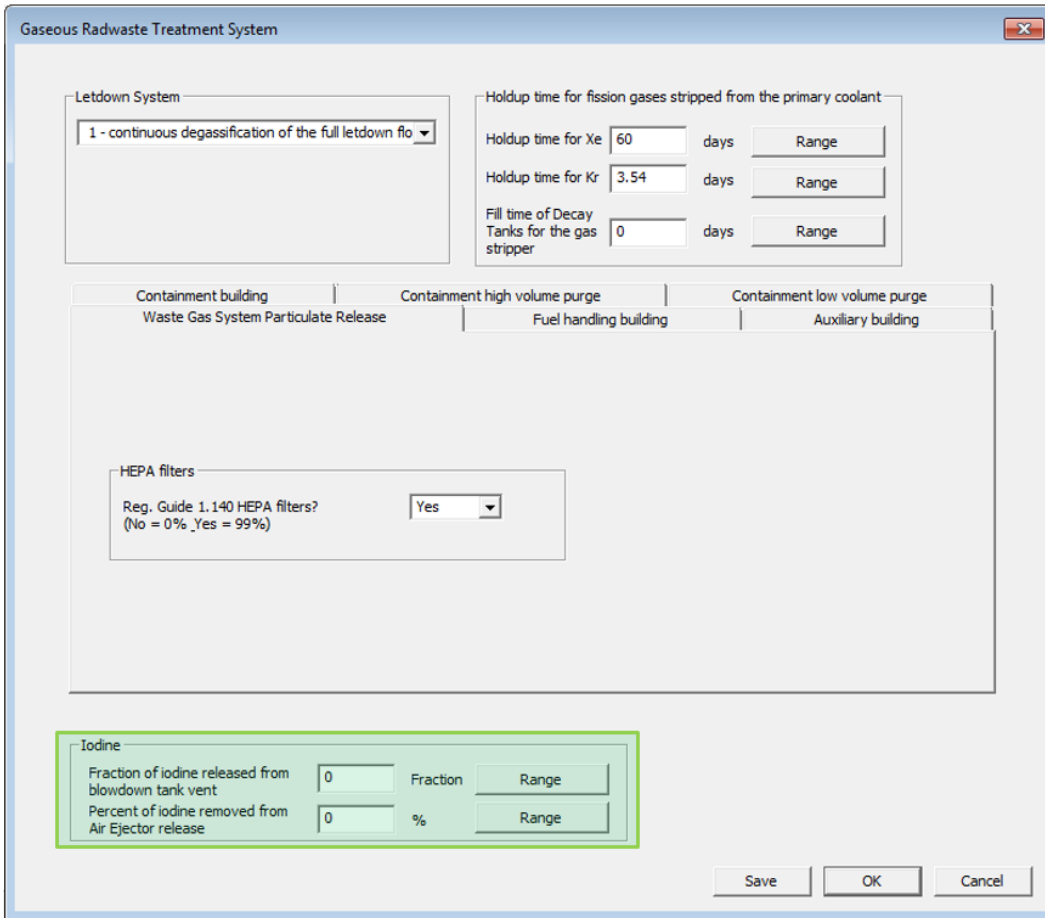
Figure 3-59 Gaseous Radwaste Treatment System Screen with Iodine field
