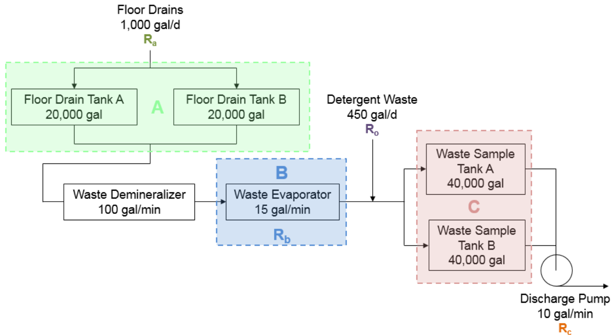
Figure 3-29 Example of liquid waste processing system flow stream scheme
