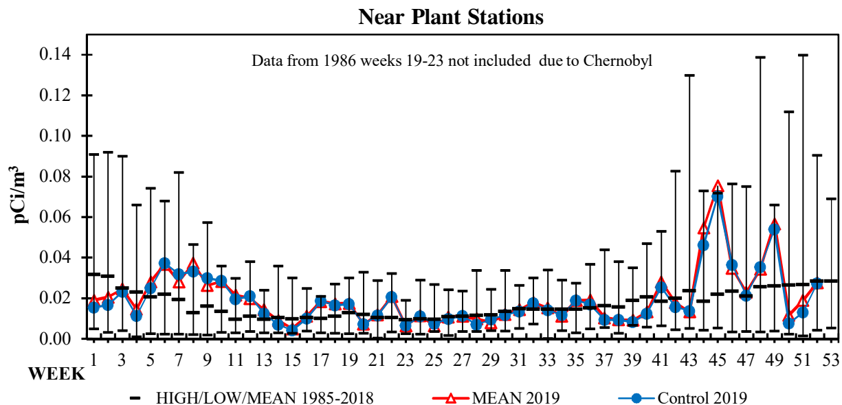
Figure 5-4 1985-2018 Weekly Hi/Low/Mean and 2019 Weekly Mean Gross Beta in Air - Near Plant Stations
