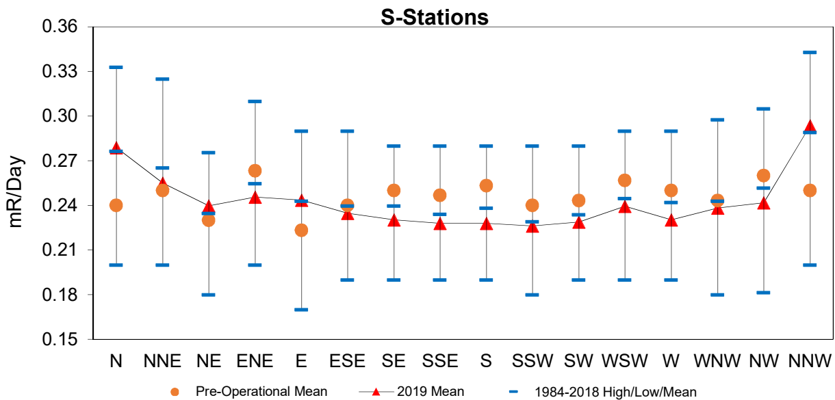
Figure 5-1 "S" Stations Quarterly TLDs 1984-2018 Hi/Low/Mean and 2019 Mean by Sector
