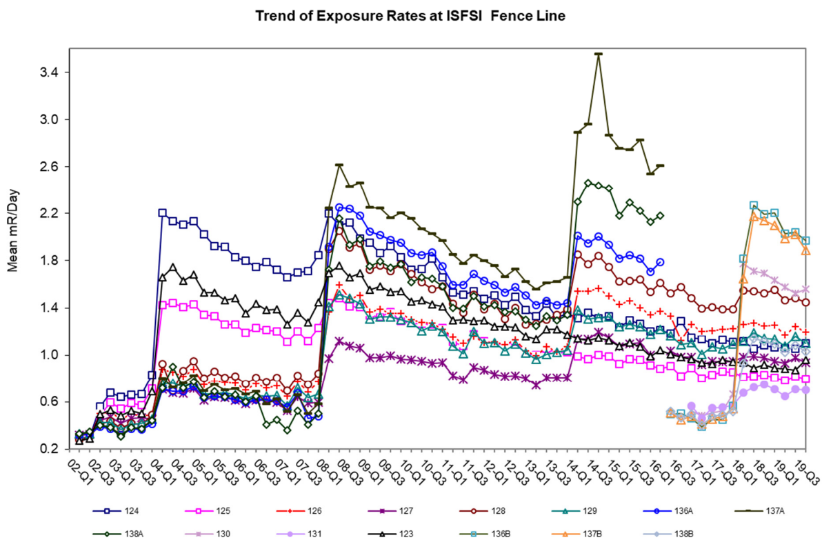
Figure 5-9 ISFSI TLD Trend at CGS
