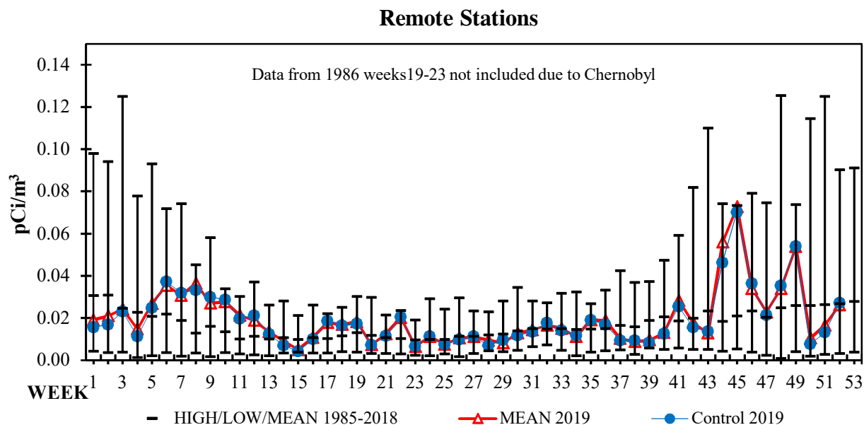
Figure 5-5 1985-2018 Weekly Hi/Low/Mean and 2019 Weekly Mean Gross Beta in Air - Remote Stations
