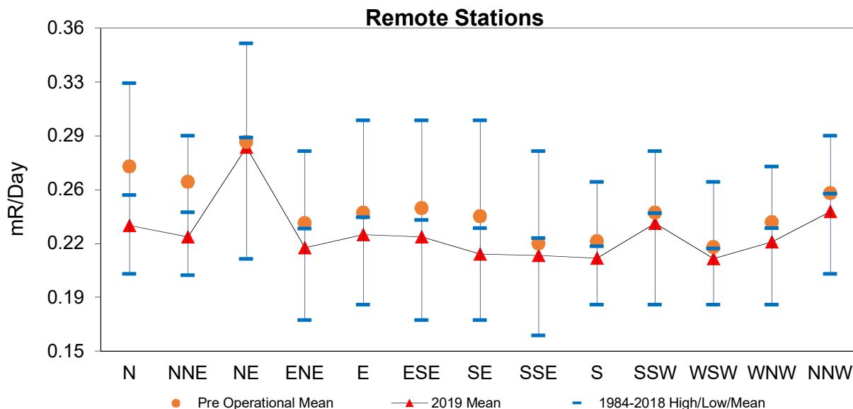
Figure 5-3 Remote Stations Quarterly TLDs 1984-2018 Hi/Low/Mean and 2019 Mean by Sector
