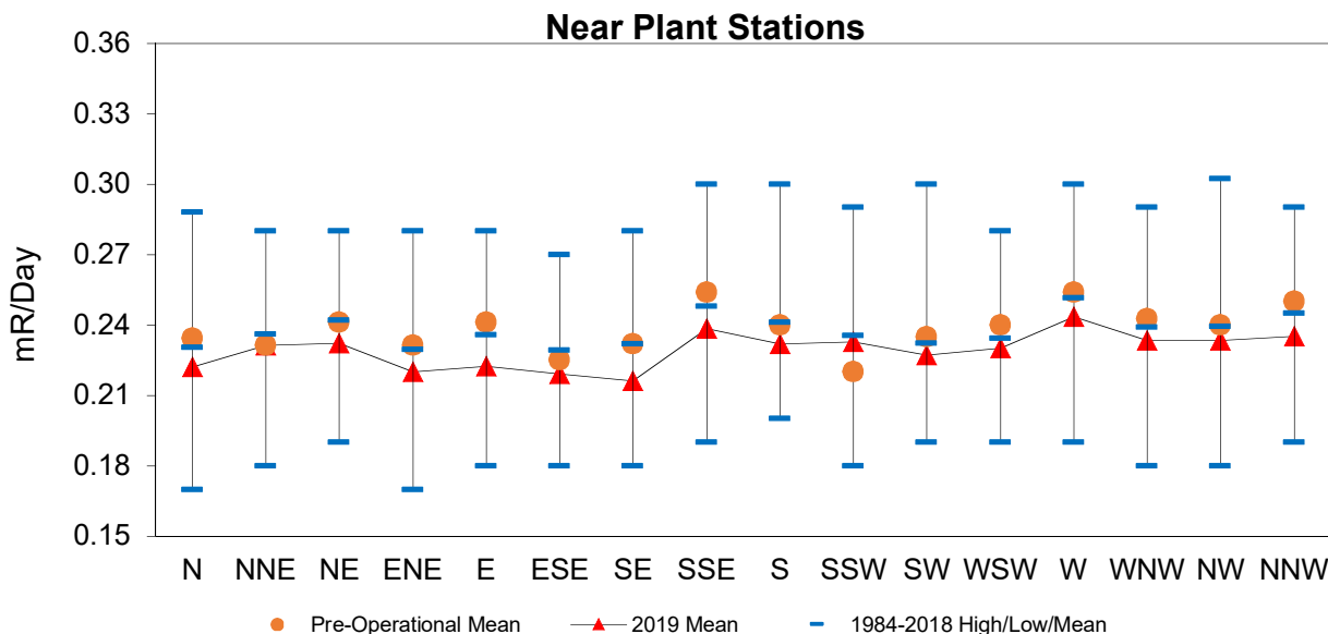
Figure 5-2 Near Plant Stations Quarterly TLDs 1984-2018 Hi/Low/Mean and 2019 Mean by Sector
