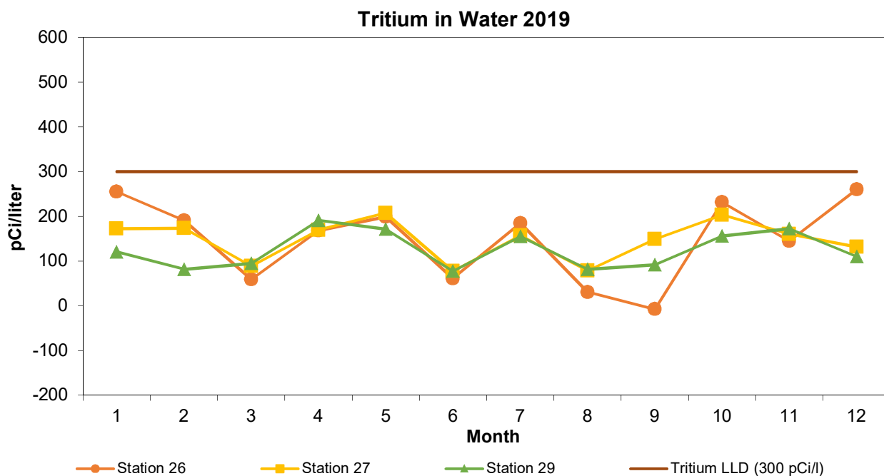
Figure 5-7 Tritium in River/Drinking (Stations 26 & 29) and Plant Discharge Water (Station 27) for 2019
