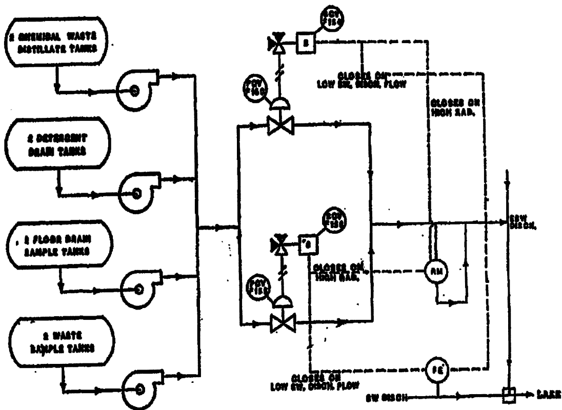
Liquid Radioactive Waste (LRW) Discharge System
