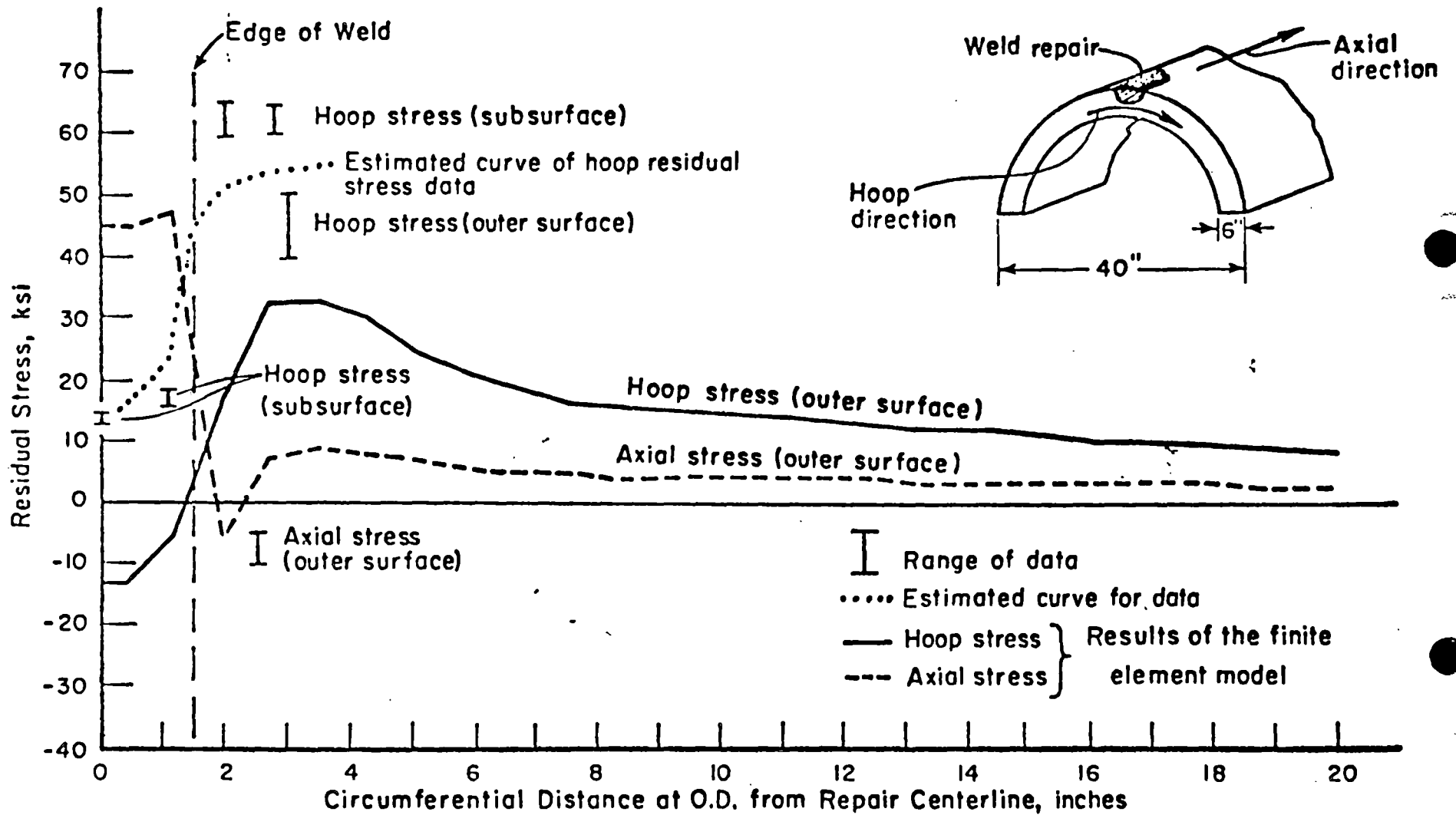
FIGURE 19. COMPARISON OF RESIDUAL STRESS DATA FOR WELD REPAIR OF HSST INTERMEDIATE VESSEL V-8 AND PRELIMINARY COMPUTATIONS BASED ON RESIDUAL STRESS MODEL
