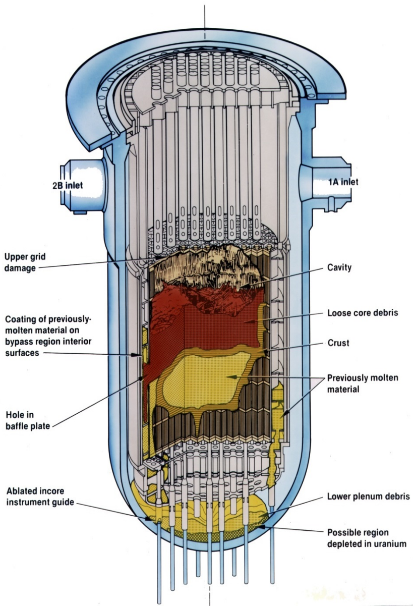
TMI-2 Core End-State Configuration. In 1988, the NRC reported the final state of the damaged TMI-2 reactor core, shown above. The accident was terminated by reflooding of the core. This action did not immediately stop further core melting, but it did prevent the core from melting through the reactor vessel.
