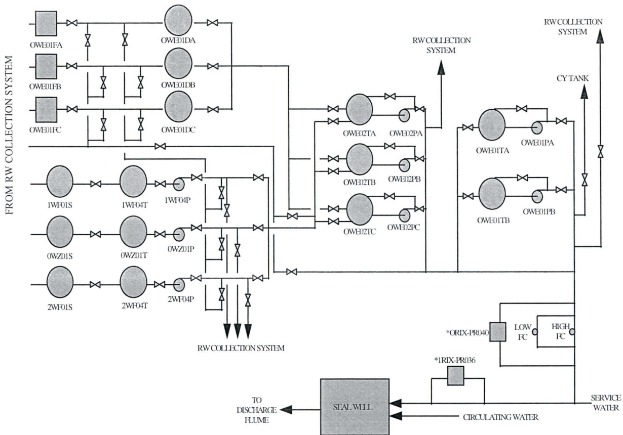
FIGURE 2-2 LIQUID RADWASTE TREATMENT SYSTEM
