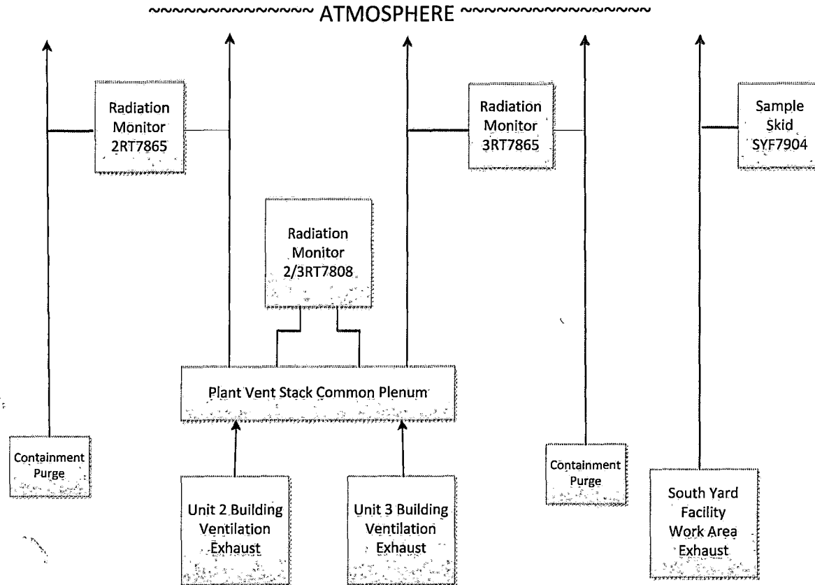
Figure 4-6 SONGS Radioactive Gaseous Waste Treatment Systems
